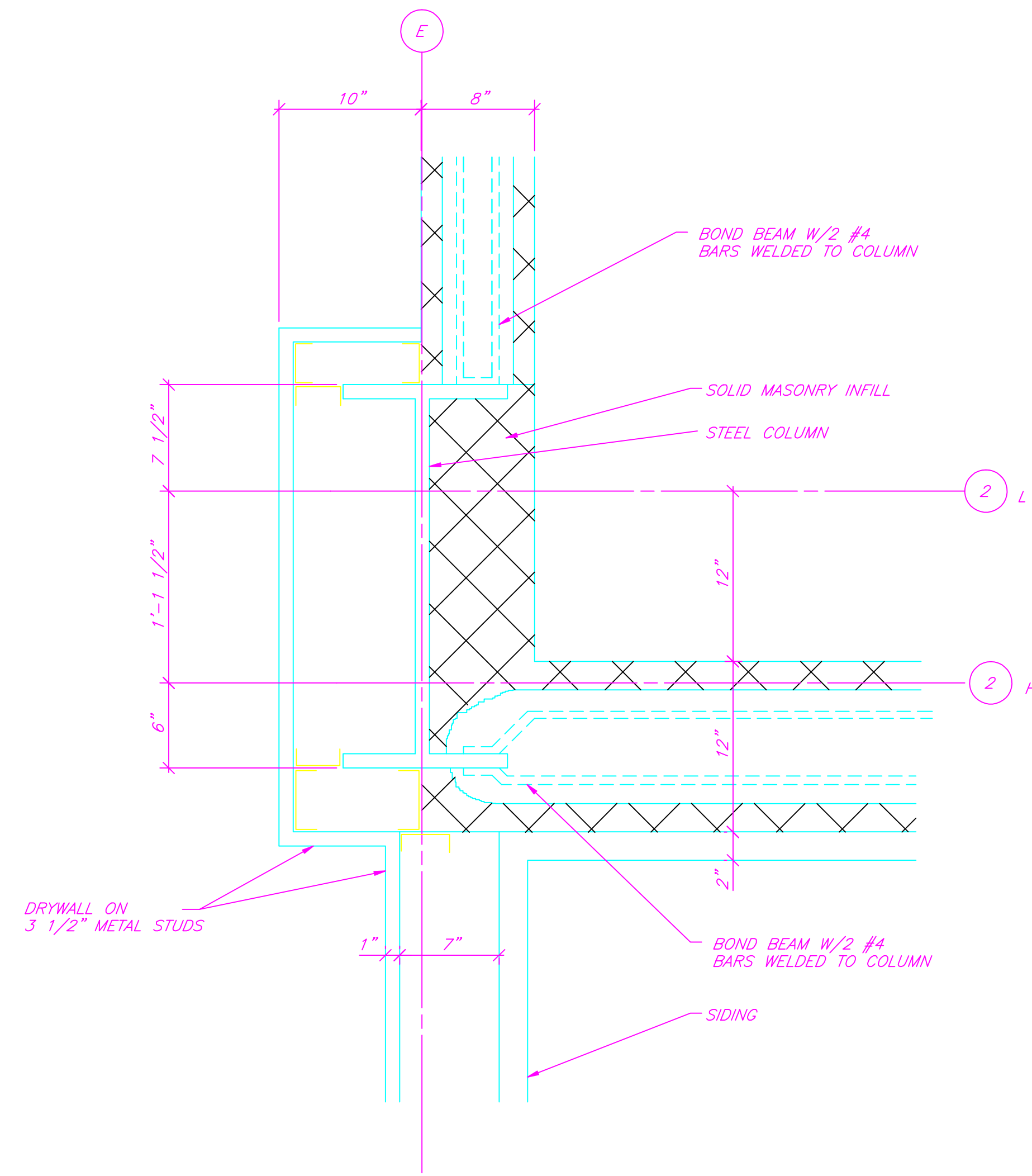
PLAN VIEW "C" OF INTERSECTION OF BOND BEAM W/ STEEL COLUMN 2E SCALE: 1 1/2"=1'-0" (INTERSECTION @ 2D OPPOSITE HAND)
