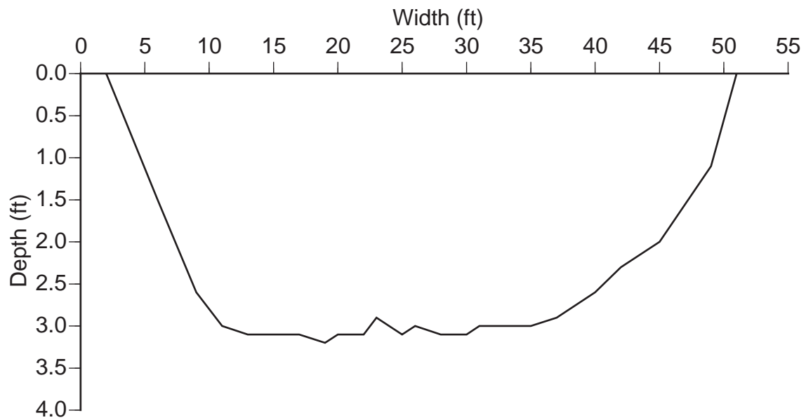
Figure 24b.—Stream channel cross-section of Dowagiac River at Sumnerville. Data from United States Geological Survey.
