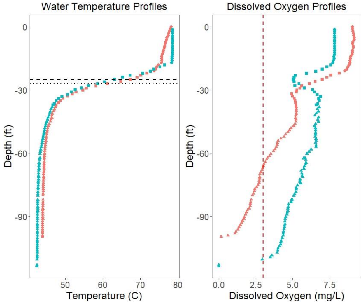
Figure 2. Temperature and dissolved oxygen profiles collected from the deepest basin of Cass Lake, collected on September 9, 2016 (orange points) and August 17, 2018 (blue points). The horizontal black dashed line represents the thermocline found August 17, 2018 and the horizontal black dotted line represents the thermocline found September 9, 2016. The vertical red line is where dissolved oxygen is at 3.0 mg/L.
