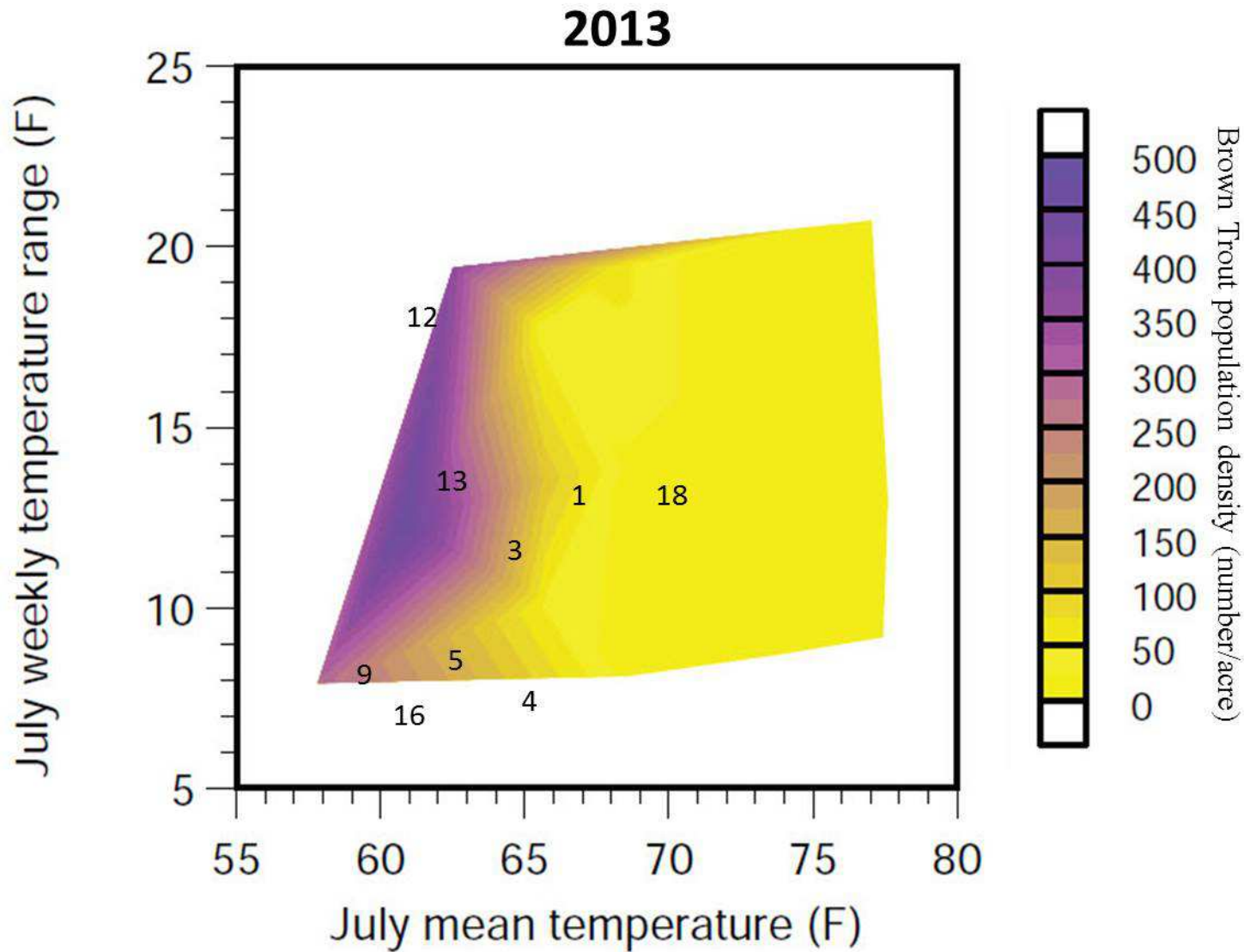
Figure 13.—Relationship between July mean water temperature, weekly temperature range, and numerical density (number/acre) of Brown Trout in Michigan streams (Zorn et al. 2009). Numbers plotted on the graph represent temperature logger deployment sites on tributaries to the Prairie River during July 2013. (See Table 3 for site locations.)
