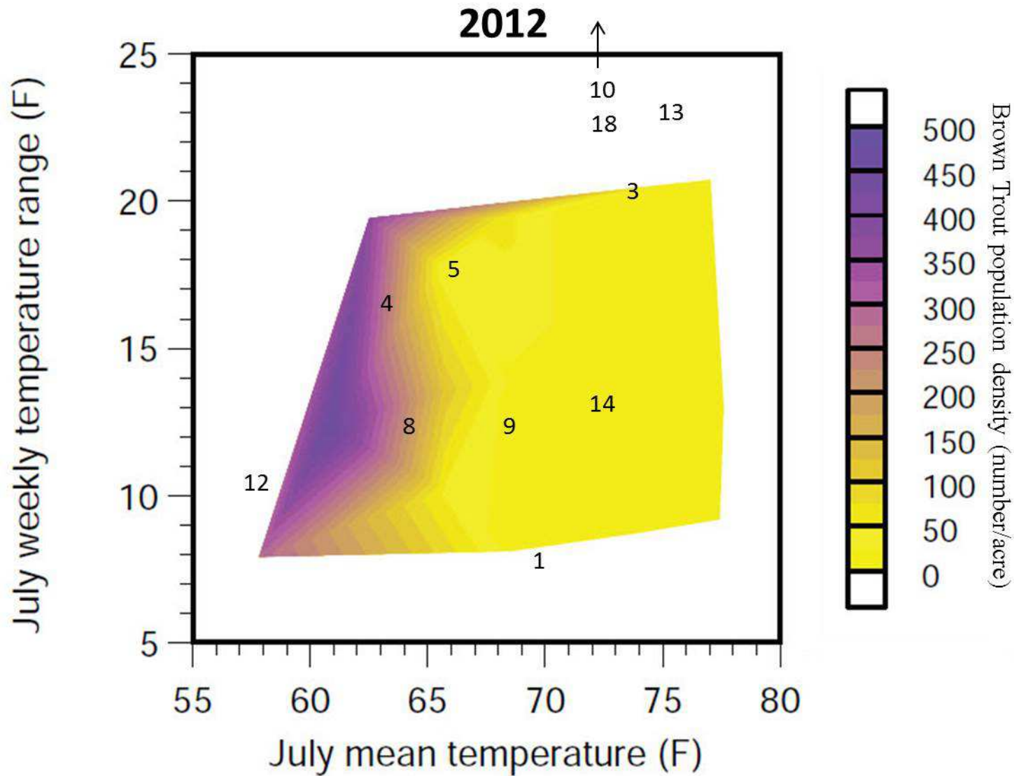
Figure 12.—Relationship between July mean water temperature, weekly temperature range, and numerical density (number/acre) of Brown Trout in Michigan streams (Zorn et al. 2009). Numbers plotted on the graph represent temperature logger deployment sites on tributaries to the Prairie River during July 2012. (See Table 3 for site locations.)
