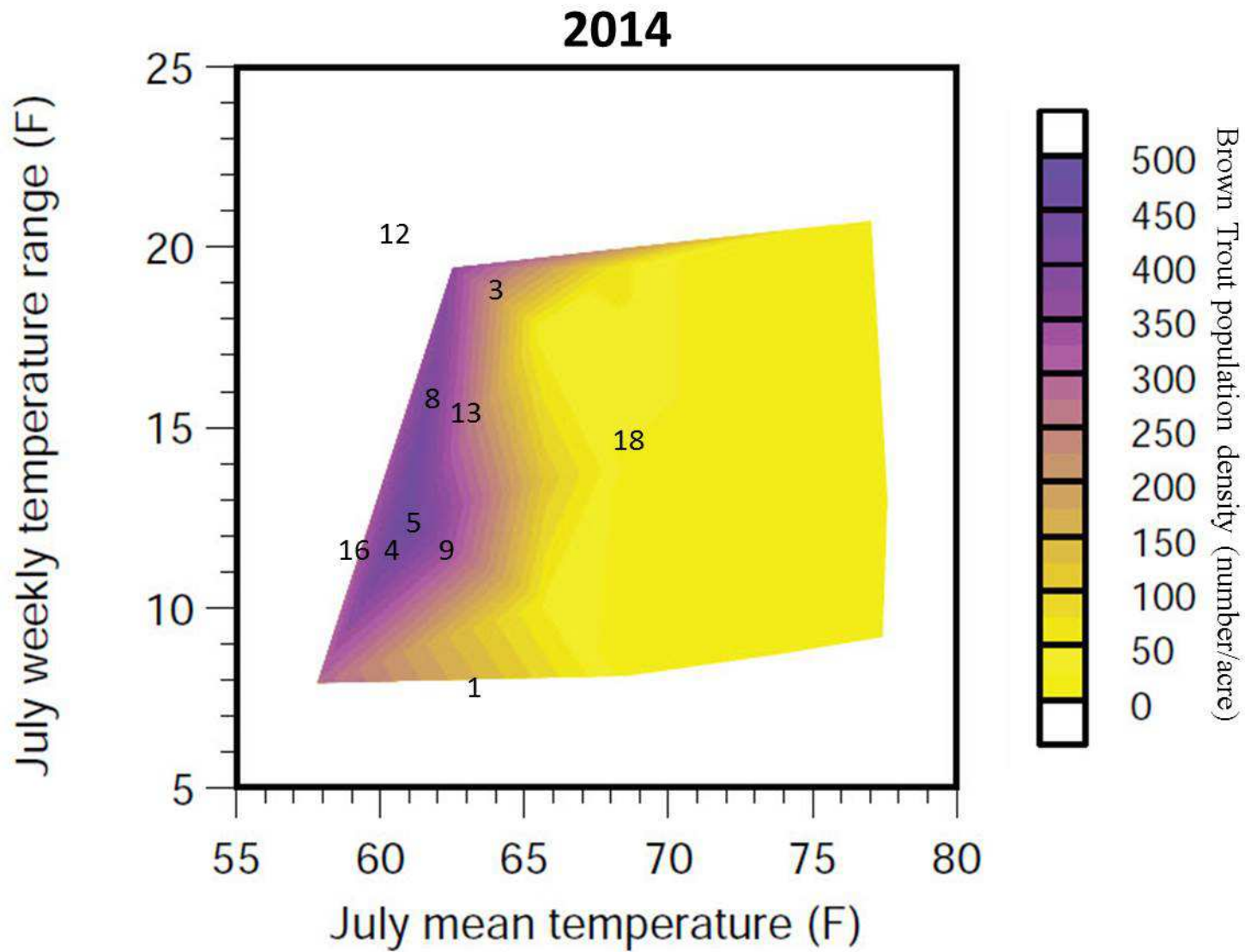
Figure 14.—Relationship between July mean water temperature, weekly temperature range, and numerical density (number/acre) of Brown Trout in Michigan streams (Zorn et al. 2009). Numbers plotted on the graph represent temperature logger deployment sites on tributaries to the Prairie River during July 2014. (See Table 3 for site locations.)
