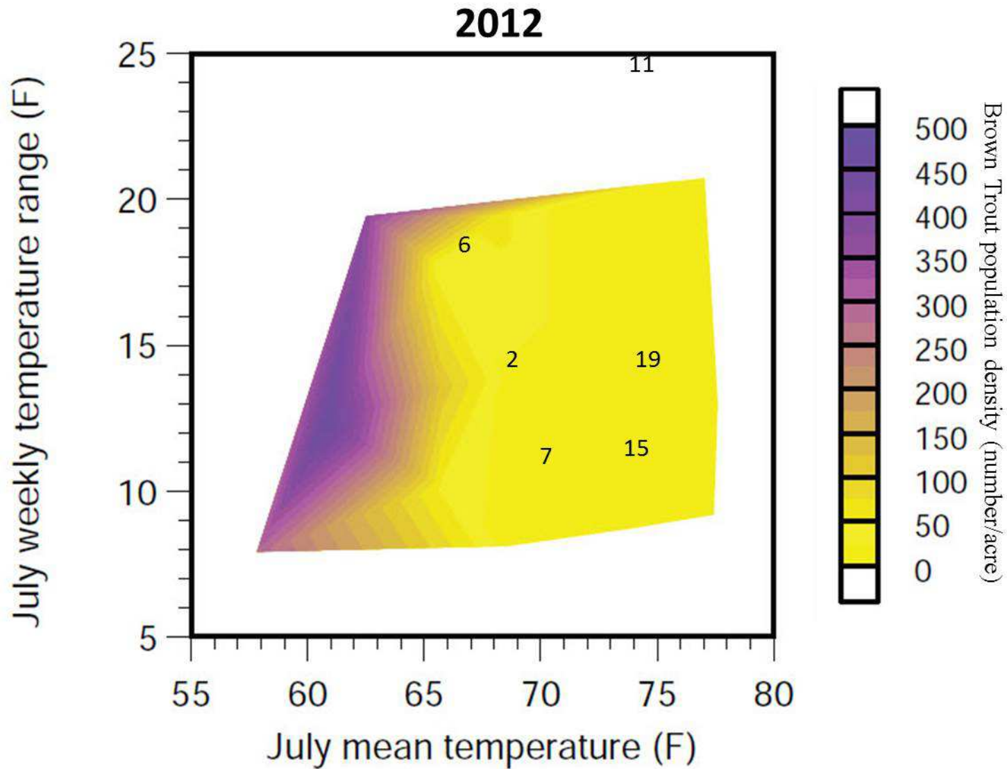
Figure 9.—Relationship between July mean water temperature, weekly temperature range, and numerical density (number/acre) of Brown Trout in Michigan streams (Zorn et al. 2009). Numbers plotted on the graph represent temperature logger deployment sites on the Prairie River during July 2012. (See Table 3 for site locations.)
