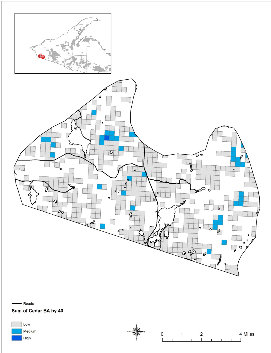
Figure 5 - Devils Creek - Chaney Lake DWC cedar analysis depicting cedar basal area by 40-acre parcels. The darker colored squares likely provide the best deer shelter potential. This analysis is based on data obtained from the USFS Forest Inventory Analysis.
