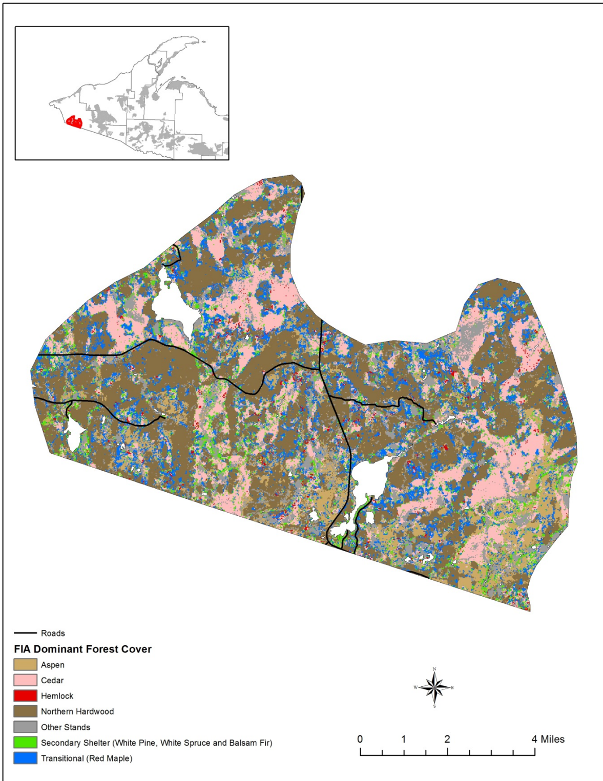
Figure 3 – The Devils Creek - Chaney Lake dominant forest cover
