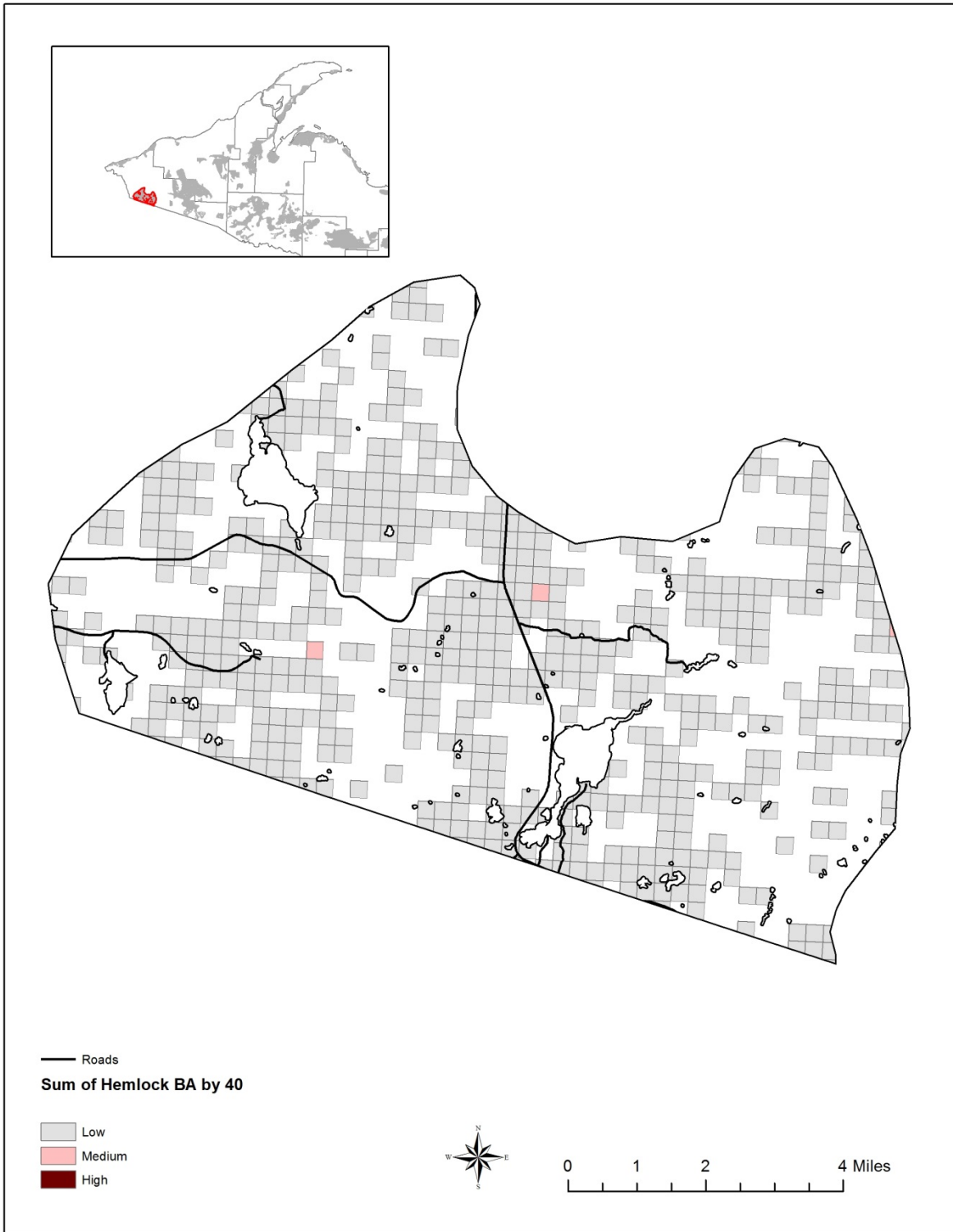
Figure 4 - Devils Creek - Chaney Lake DWC hemlock analysis depicting hemlock basal area by 40-acre parcels. The darker colored squares likely provide the best deer shelter potential. This analysis is based on data obtained from the USFS Forest Inventory Analysis.
