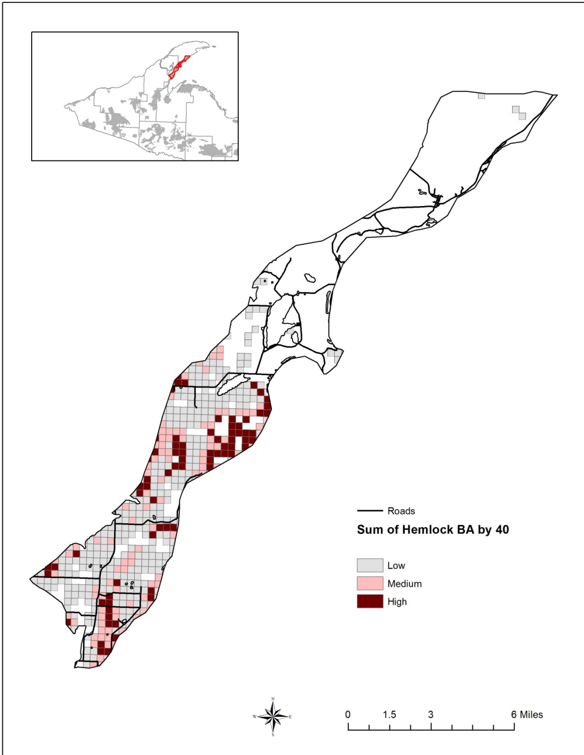
Figure 4 - East Keweenaw DWC hemlock analysis depicting hemlock basal area by 40-acre parcels. The darker colored squares likely provide the best deer shelter potential. This analysis is based on data obtained from the USFS Forest Inventory Analysis.
