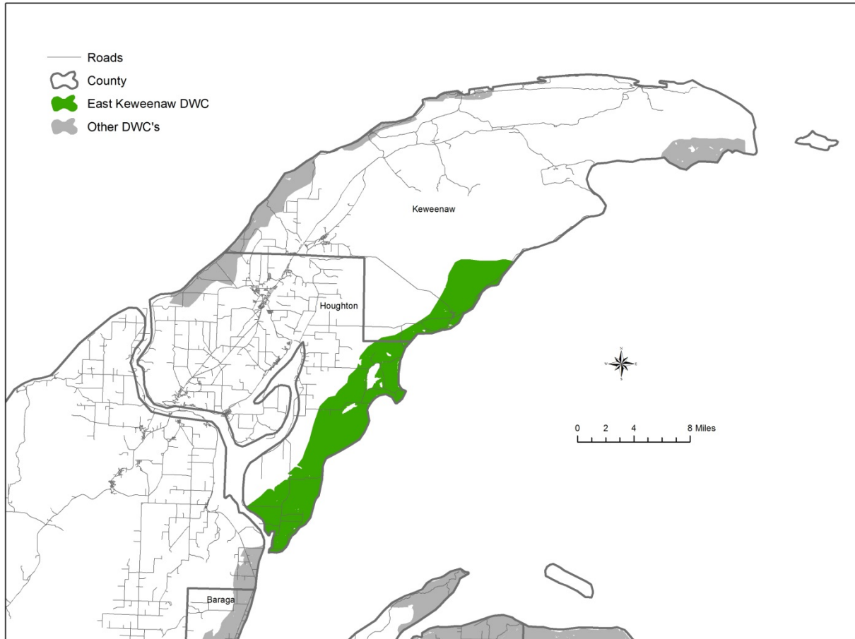
Figure 1 – Keweenaw Peninsula DWC map with the East Keweenaw Deer Wintering Complex in green.
