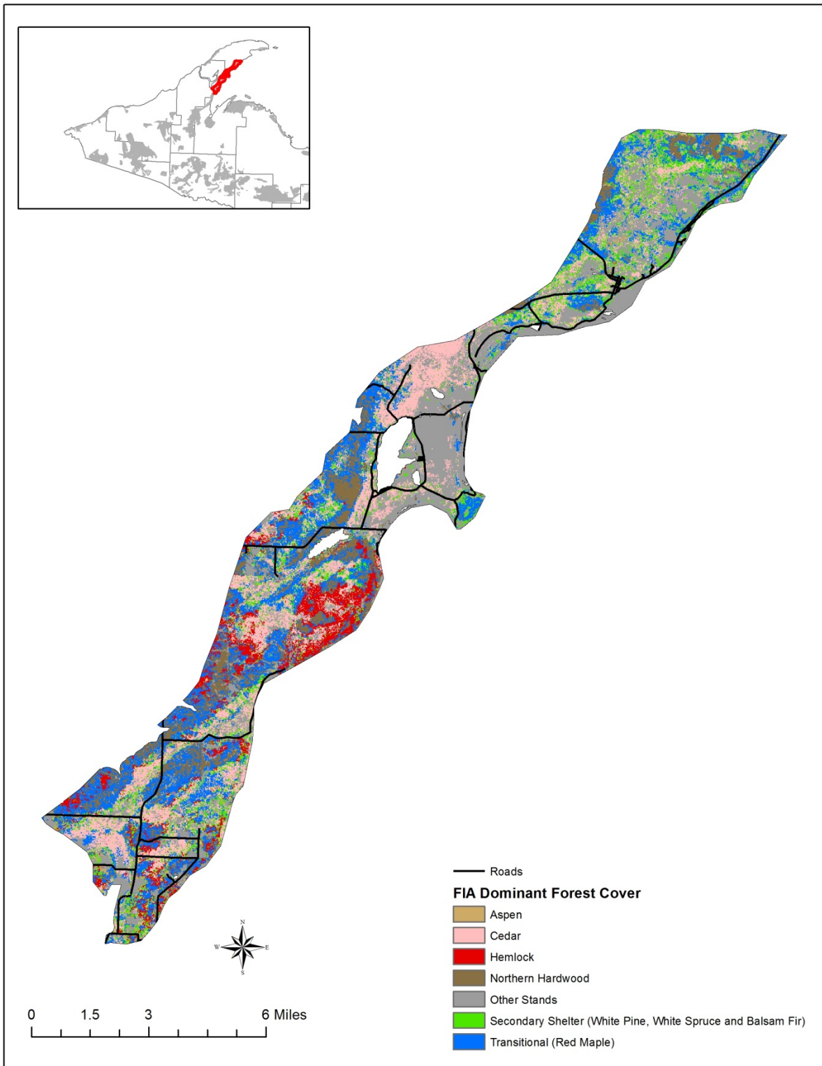
Figure 3 – The East Keweenaw dominant forest cover
