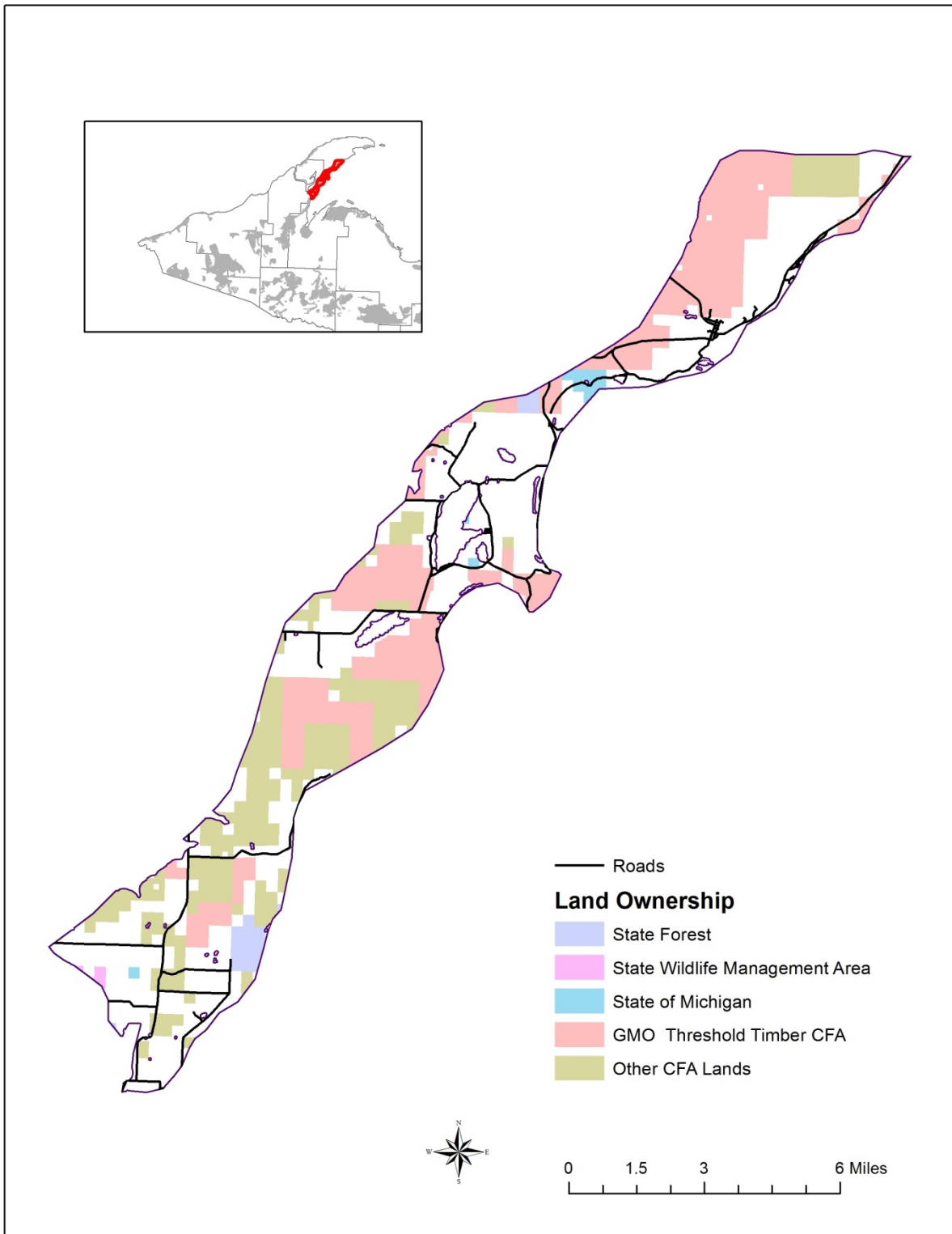
Figure 2 - East Keweenaw DWC ownership map.
