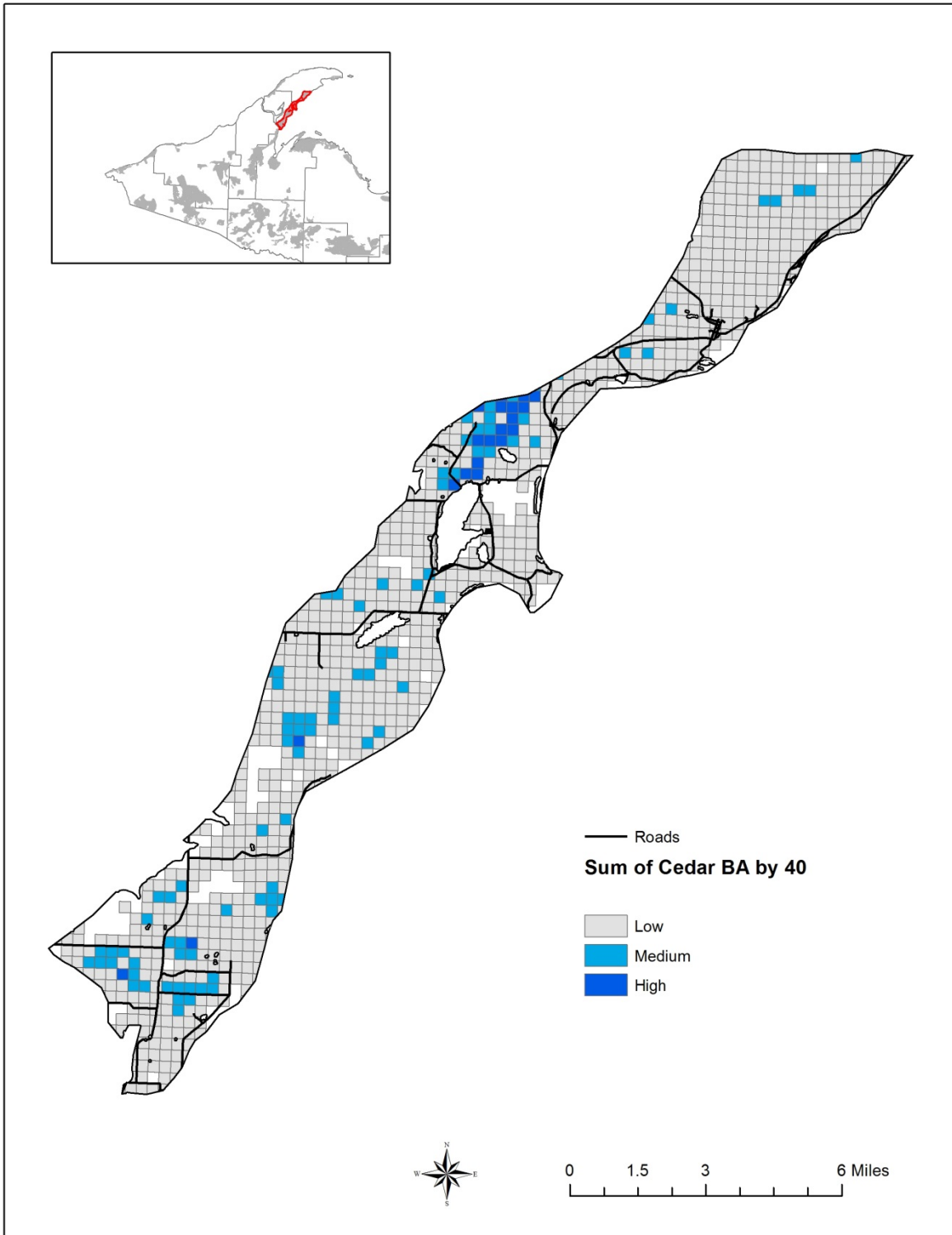
Figure 5 - East Keweenaw DWC cedar analysis depicting cedar basal area by 40-acre parcels. The darker colored squares likely provide the best deer shelter potential. This analysis is based on data obtained from the USFS Forest Inventory Analysis.
