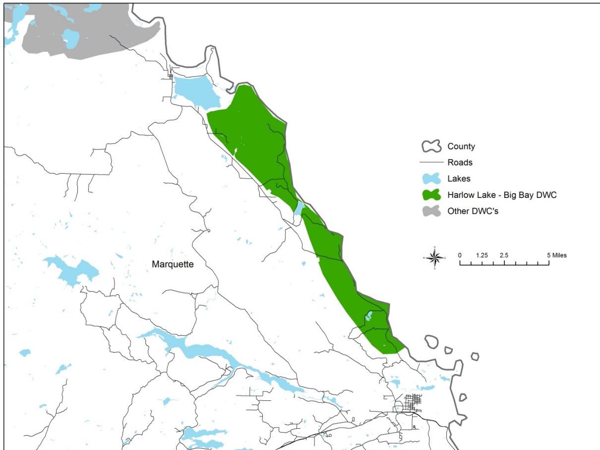
Figure 1 – Central UP DWC map with the Harlow Lake - Big Bay Deer Wintering Complex in green.
