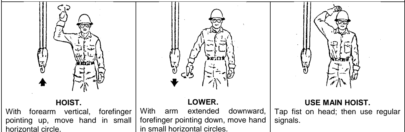
Figure 1 Standard Hand Signals for Controlling Crane Operations
