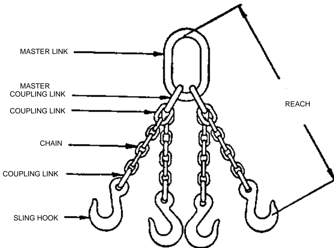
FIGURE 3 MAJOR COMPONENTS OF A QUADRUPLE SLING
