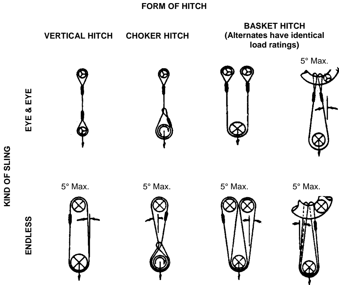
FIGURE 4 BASIC SLING CONFIGURATIONS WITH VERTICAL LEGS
