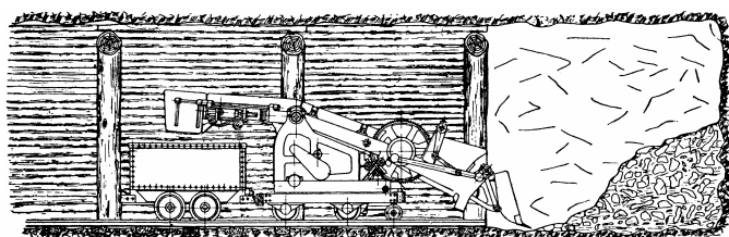
SHOWING PROPORTIONS—HALBY SHOVELING MACHINE IN 8x8 FT. DRIFT
