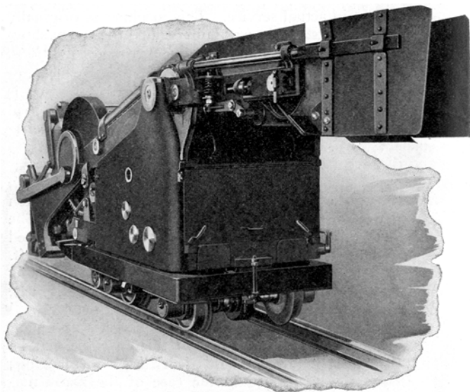
REAR VIEW—HALBY SHOVELING MACHINE
