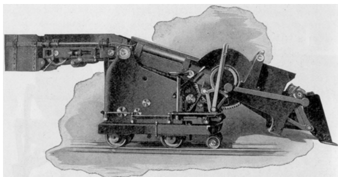
SIDE VIEW—HALBY SHOVELING MACHINE
