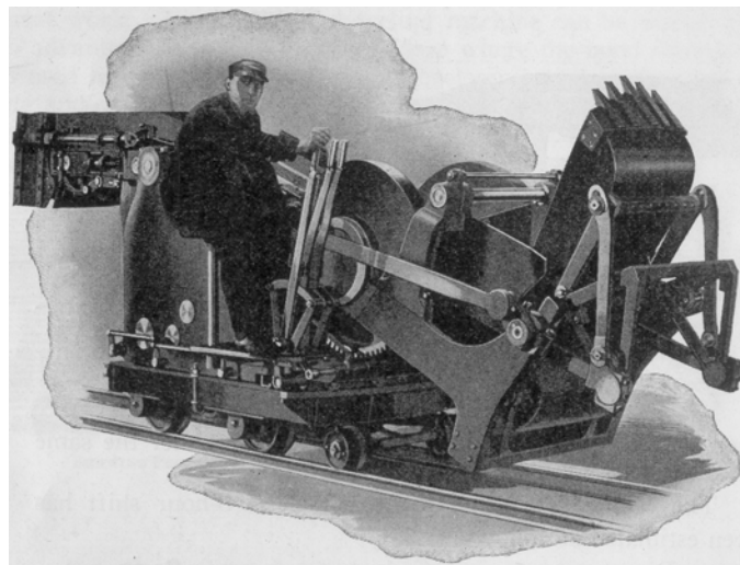
HALBY SHOVELING MACHINE—SHOWING DUMPING POSITION OF SHOVEL
