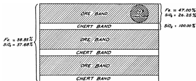
FIG. 1. IDEAL STRUCTURE OF HARD CHERTY ORE SHOWING ALTERNATE BANDS OF SILICEOUS IRON OXIDE AND NEARLY PURE CHERTY SILICA
