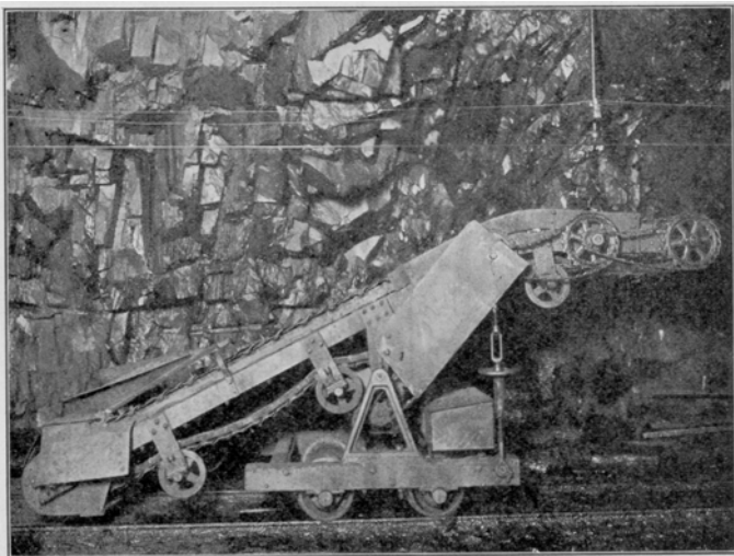
PORTABLE LOADER AT THE NORTH LAKE MINE OF THE CLEVELAND-CLIFFS IRON CO., ISHPEMING, MICH.
