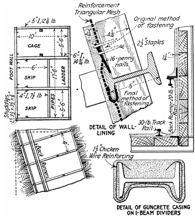
FIGURE 1. SHAFT ARRANGEMENT AND DETAIL OF COATED MEMBERS
