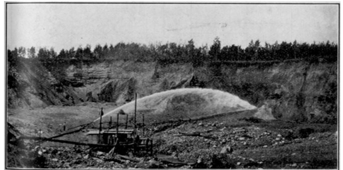
HYDRAULIC METHOD OF STRIPPING OVERBURDEN
