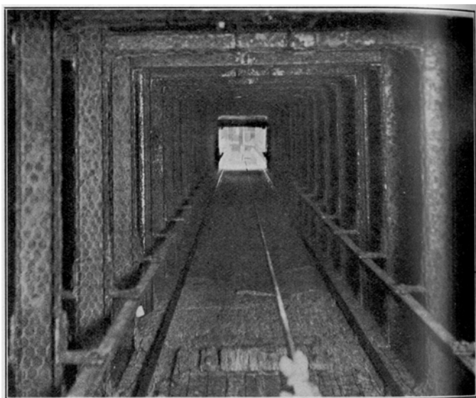
VIEW LOOKING UP "A" SHAFT SHOWING COMPLETED GUN-CRETE WORK ABOVE. REINFORCING SET BELOW BUT NOT CONCRETED YET
