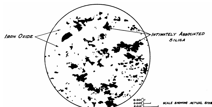
FIG. 2 PHOTOMICROGRAPH OF ORE-BAND SHOWING INTIMATELY ASSOCIATED SILICA NO SILICA VISIBLE TO NAKED EYE MAGNIFIED 45 DIAM. IRON 47.00% INTIMATELY ASSOCIATED SILICA 26.25% DRIED AT 212°F.
