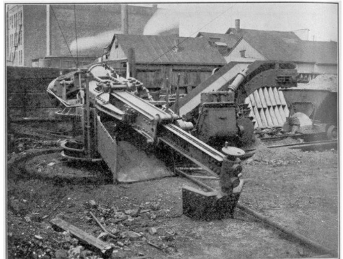
BILLINGS AND MIDDLEMISS SHOVELING MACHINE
