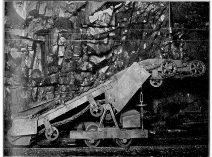
PORTABLE LOADER, INSTALLED TO FACILITATE THE LOADING AND DISPOSAL OF ROCK
