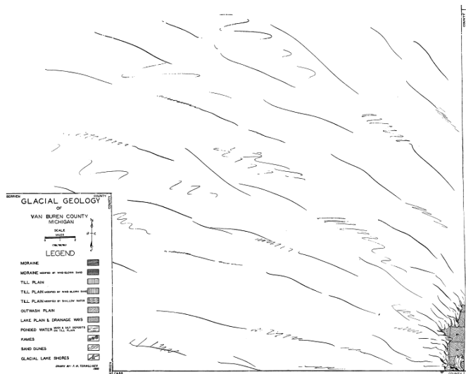
Figure 9. First stage of glacial retreat in Van Buren County.
