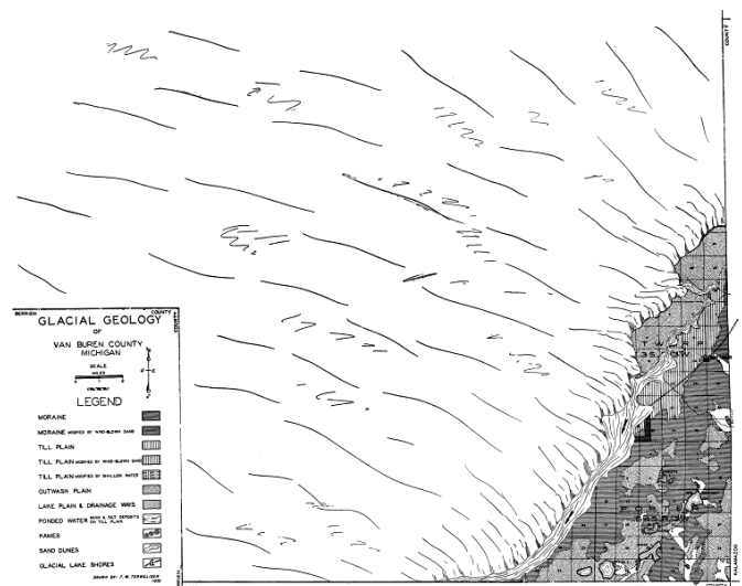
Figure 12. Fourth stage of glacial retreat in Van Buren County.
