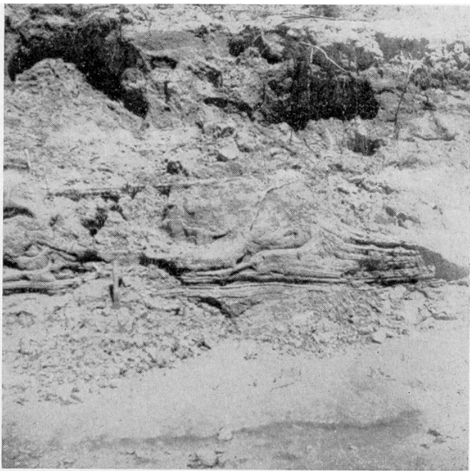
Figure 21. Another view of the two layers of varves in roadside ditch in the southeast quarter of section 21, South Haven Township.
