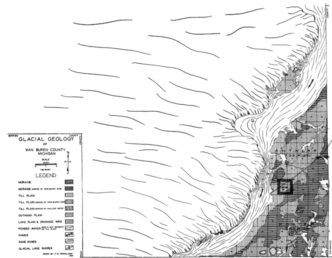
Figure 13. Fifth stage of glacial retreat in Van Buren County.
