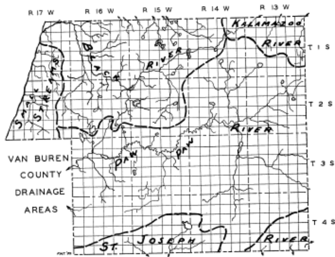
Figure 2. Van Buren County drainage areas.
