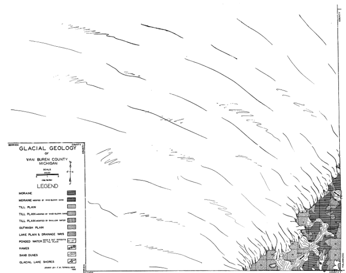
Figure 11. Third stage of glacial retreat in Van Buren County.
