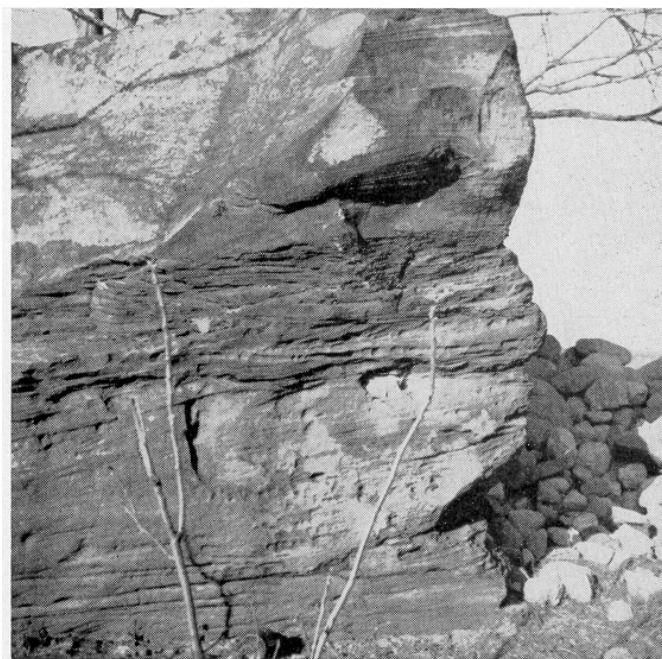
Figure 4. Close-up of Marshall boulder. This view shows the cross-bedding which is characteristic of much of the Marshall sandstone. Notice how the effects of weathering have heightened the details and pitted the surface of the rock.
