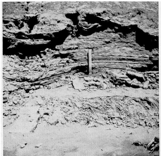
Figure 20. Two sets of varves shown in deposit along ditch on north side of road between sections 21 and 28, South Haven Township. The lower set of varves was deposited in a lake formed in front of the ice which had retreated into the Lake Michigan basin following Valparaiso time. These varves were crumpled under the foot of the ice as it advanced to the position of the Lake Border Moraine. The upper set of varves was deposited in the waters of Lake Glenwood following Lake Border time. Elsewhere in this exposure the two layers of varves are separated by a small amount of till.
