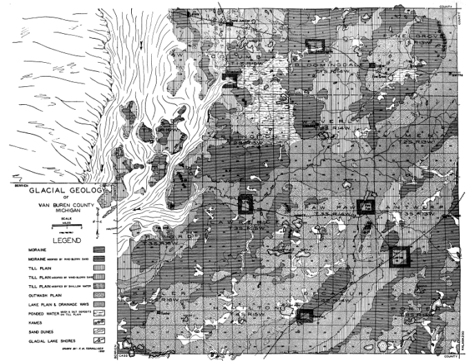
Figure 19. Eleventh stage of glacial retreat in Van Buren County.
