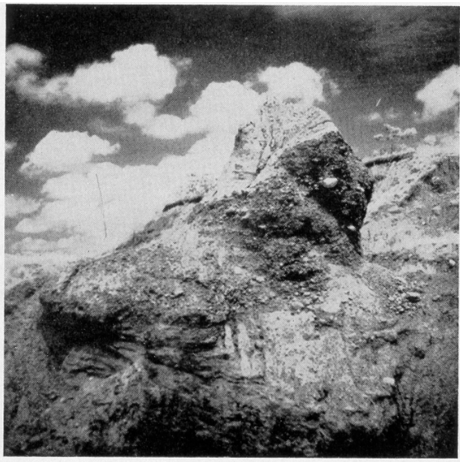
Figure 6. A pinnacle of "crag" in the bottom of a gravel pit north of Hartford. This view shows the great variation in size of pebbles and stones in the beds.
