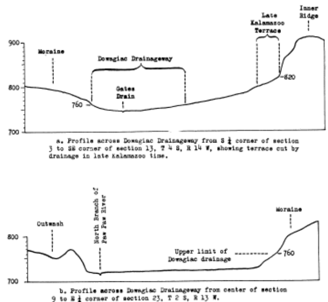
Figure 8. Profiles across Dowagiac Drainageway.
