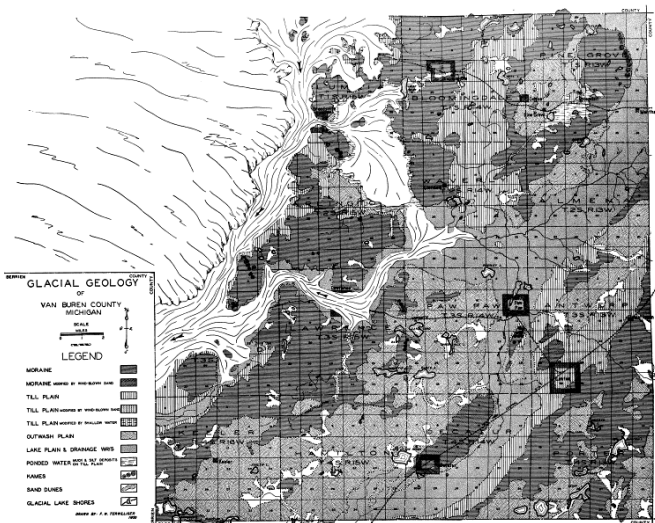
Figure 18. Tenth stage of glacial retreat in Van Buren County.
