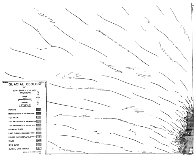
Figure 10. Second stage of glacial retreat in Van Buren County.
