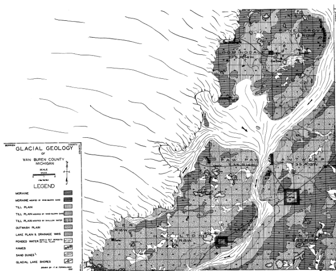
Figure 16. Eighth stage of glacial retreat in Van Buren County.
