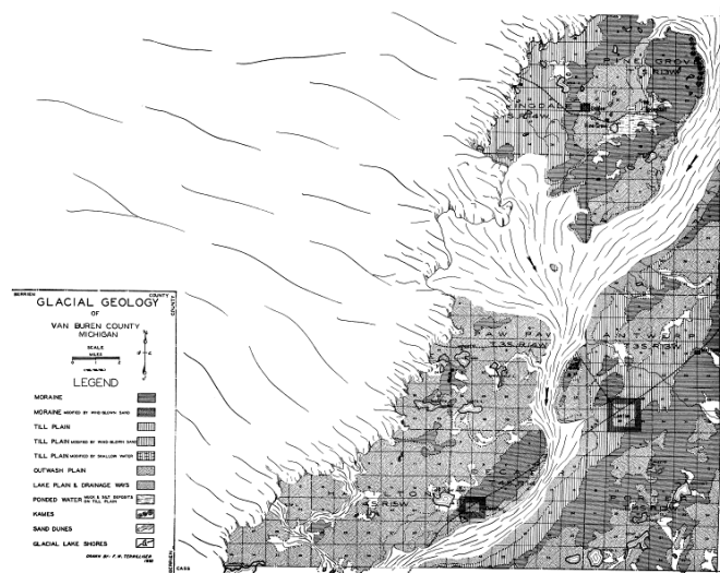
Figure 15. Seventh stage of glacial retreat in Van Buren County.
