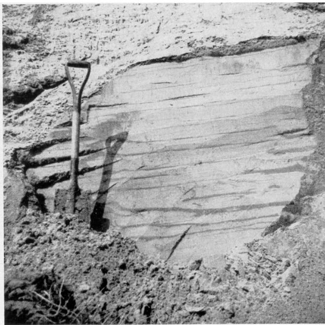
Figure 22. Seasonally banded sand in the Lake Glenwood embayment in section 6, Geneva Township. The dark streaks are sand containing iron oxides and organic material which were flocculated and deposited during the winter. Where the face of the sand pit has been exposed to wind action, the looser summer sand has been blown away, and the better cemented or more coherent winter layers are festooned at the edges.
