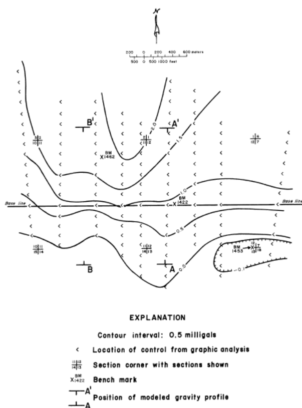
Figure 9. Gravity residual – 1, anomaly caused by deep body.
