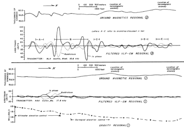
Figure 12. Composite geophysical profiles along regional lines 1 and 3.
