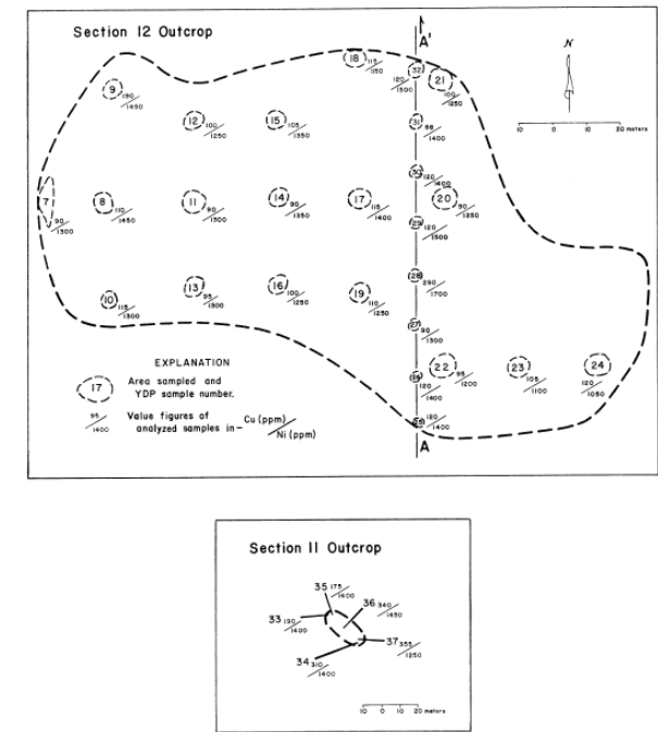
Figure 2. Location of analyzed samples. See Figure 3 for locations
