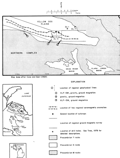
Figure 1. Yellow Dog Plains general regional geology and location.
