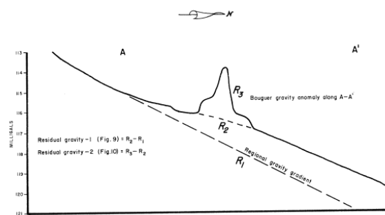
Figure 8. Gravity profile along A – A', showing how residual gravity anomalies were determined.
