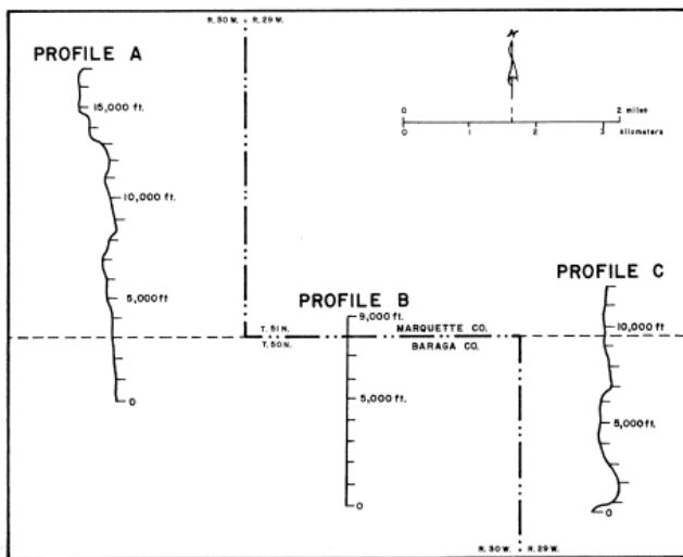
Figure 13. Location of geochemical soil profiles.
