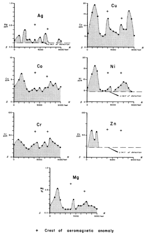
Figure 15. Geochemical profiles in soil along profile B.
