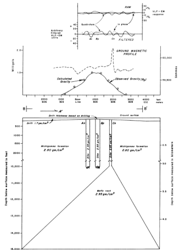
Figure 11b. Composite geophysical profiles and geologic model
