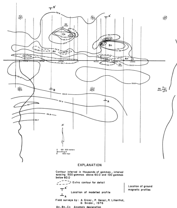
Figure 4. Ground magnetics of detailed study area.
