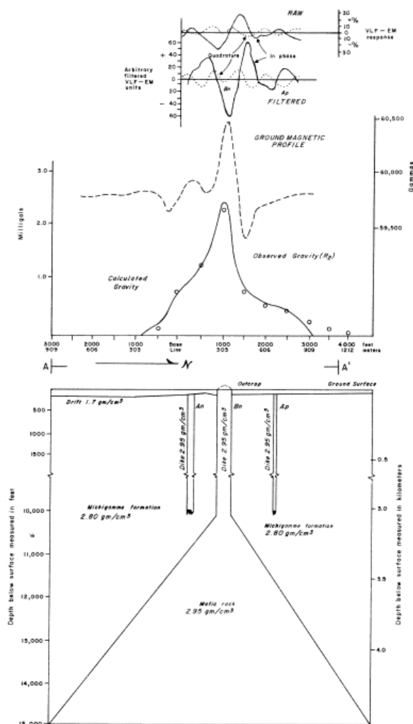
Figure 11a. Composite geophysical profiles and geologic model
