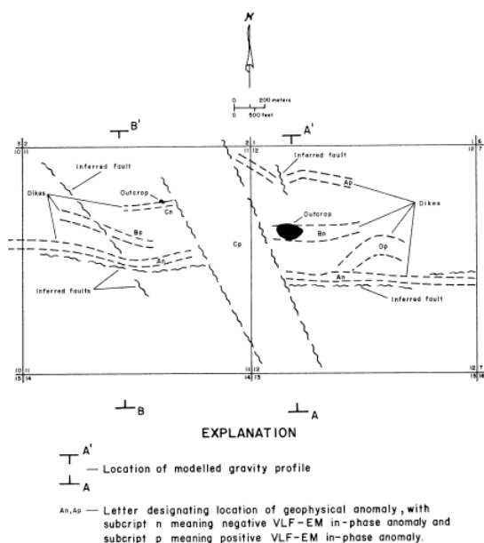
Figure 7. Geology of the detailed study area inferred from geophysical surveys.
