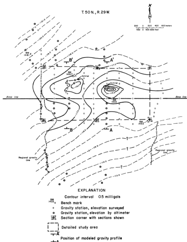
Figure 3. Complete Bouguer gravity anomaly.
