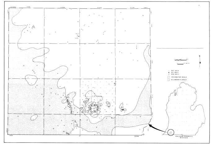
Figure 6. Bedrock Geology of Cass County, Michigan.
