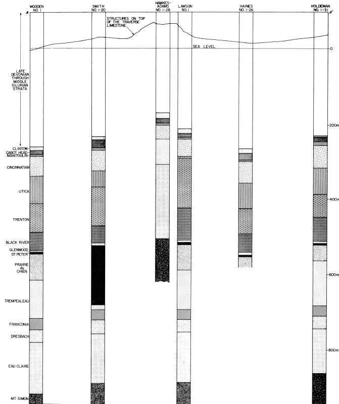
Figure 5. Generalized geologic cross-section and profile of Traverse Limestone tops, Calvin 28 cryptoexplosive disturbance.
