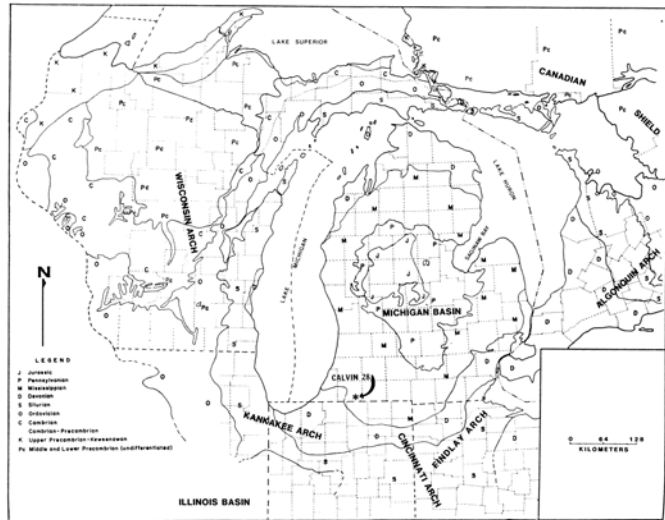
Figure 3. The Michigan Basin and surrounding geologic structures (modified from Stonehouse, 1969).
