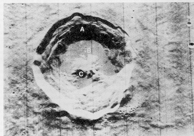
Lunar Orbiter image of the crater Bërg; 45°N, 28°E; northeast region of the Moon (Schultz, 1976).
