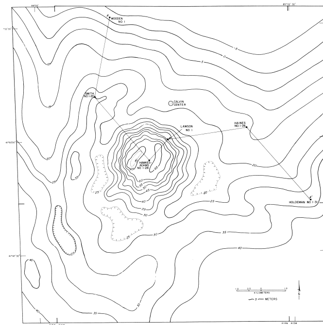
Figure 2. Traverse Limestone structure contour map and line of geologic cross-section, Calvin 28 cryptoexplosive disturbance.
