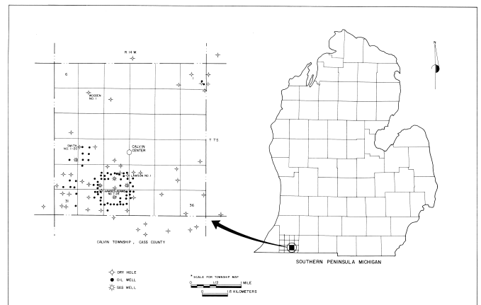
Figure 1. Location of study area, Calvin 28 cryptoexplosive disturbance, Cass County, Michigan.
