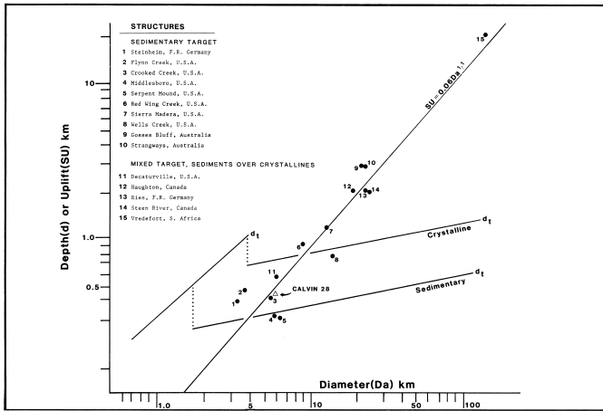
Figure 9. The Calvin 28 cryptoexplosive disturbance compared with stratigraphic uplift/diameter relationships for terrestrial impact structures (modified from Grieve and others, 1981).
