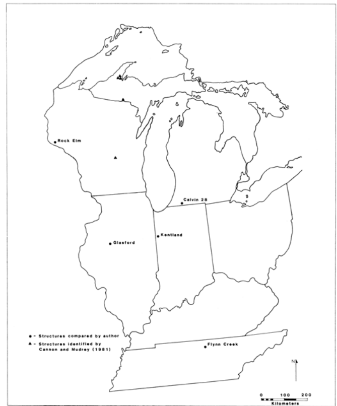
Figure 8. Location of selected Midwestern cryptoexplosive disturbances.
