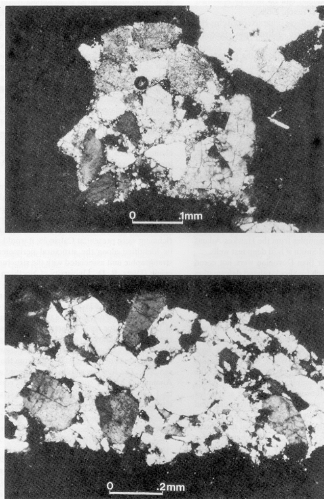
Figure 7. Photographs illustrating microscopic breccia from the Calvin 28 cryptoexplosive disturbance: Lawson #1, 1016.5-1018 m.
