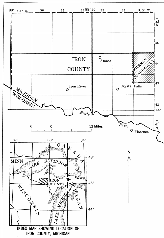
FIGURE 1.—Index map showing location of Kiernan quadrangle, Iron County, Mich.
