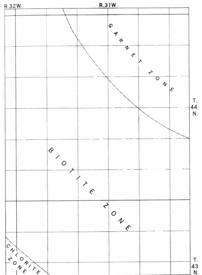
FIGURE 4.—Outline map of Kiernan quadrangle showing approximate location and trends of metamorphic zones.
