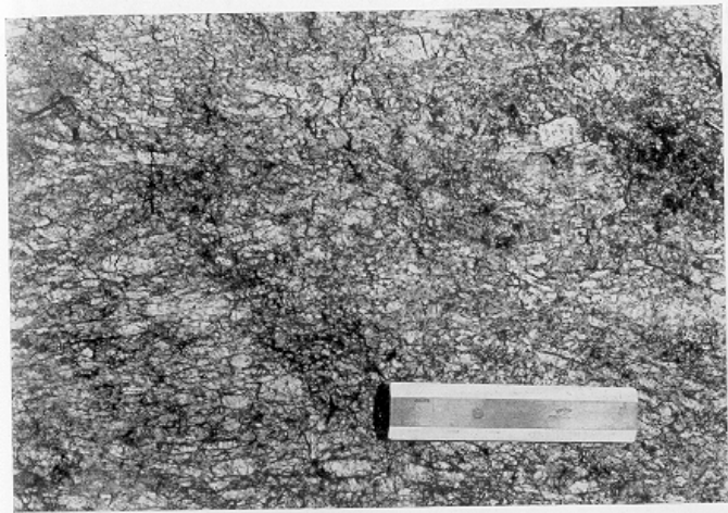
FIGURE 5.—Foliated inequigranular granitic rock of Margeson Creek gneiss. Large tabular feldspars are well aligned and form about 50 per cent of the rock. Loc. 3,600 feet north and 1,300 feet west of southeast corner sec. 12, T. 44 N., R. 32 W. Length of scale is 6 inches.
