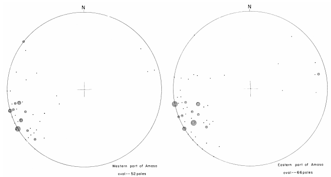
FIGURE 19.—Poles of foliation planes in Margeson Creek gneiss. Plotted on lower hemisphere of equal-area projection. Circles around points represent more than one pole at same point. Western part of Amasa oval—52 poles. Eastern part of Amasa oval—66 poles.
