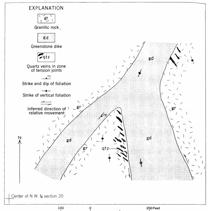
FIGURE 20.—Diagrammatic plan view showing relationships of granitic rock, basic dikes, quartz veins, and inferred fault in the southwestern part of the NE \frac{1}{4} NW \frac{1}{4} sec. 20, T. 44 N., R. 31 W.
