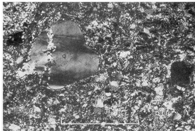
FIGURE 16.—Photomicrograph of metarhyolite from Hemlock formation, 550 feet north and 1,650 feet west of the southeast corner, sec 33, T. 44 N., R. 31 W. Embayed quartz “eye” phenocryst has strain shadows. Groundmass contains fine-grained quartz and sericite and abundant spherulites, probably of feldspar. Crossed nicols. (q) quartz, (ser) sericite, (sp) spherulite.
