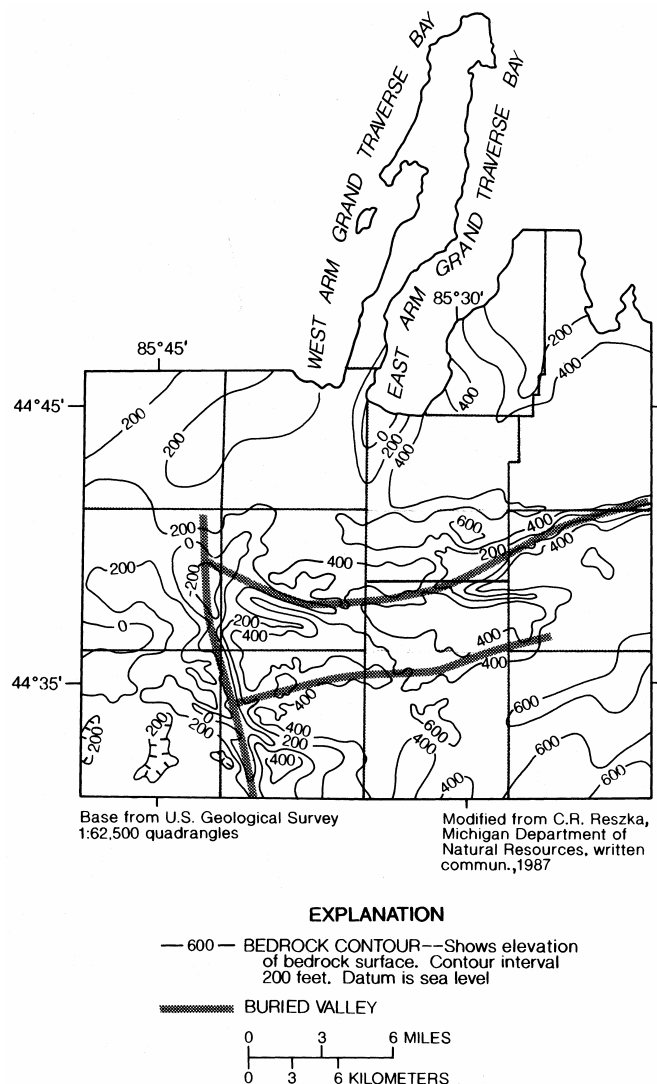
Figure 5.--Buried valleys and configuration of the bedrock surface.
