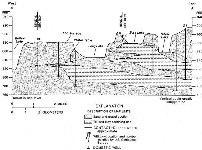
Figure 9.--Relation of till and clay confining units to sand and gravel aquifers near Long, Bass, and Silver Lakes. (Line of section shown on plate 1.)
