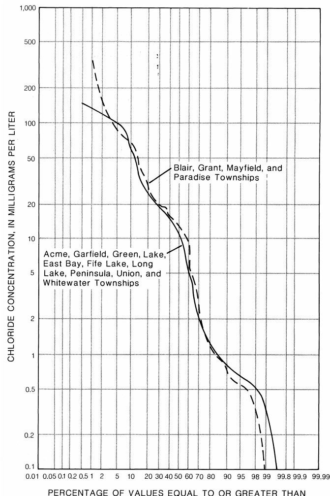
Figure 19.--Frequency distribution of chloride concentrations in ground water.
