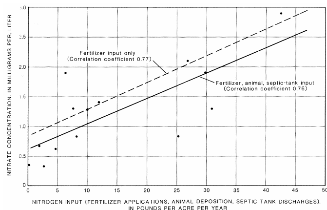
Figure 18.--Relation of nitrate concentrations of ground water to nitrogen input.
