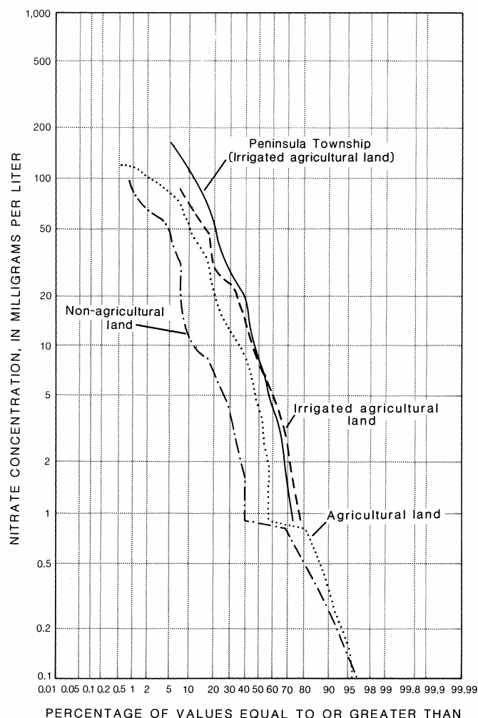
Figure 17.--Frequency distributions of nitrate concentrations in ground water from non-agricultural land, agricultural land, irrigated agricultural land, and irrigated agricultural land in Peninsula Township.
