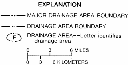
Figure 8.--Drainage areas.
