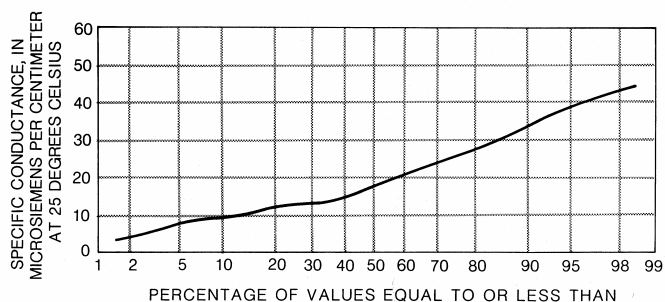
Figure 12.--Frequency distributions of specific conductance and pH of precipitation near Kingsley.
