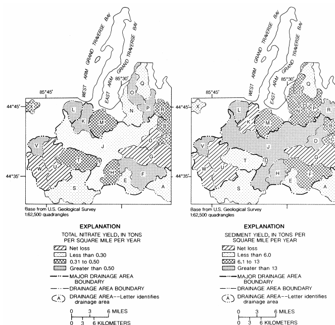
Figure 15.--Nitrate and sediment yields by drainage area.
