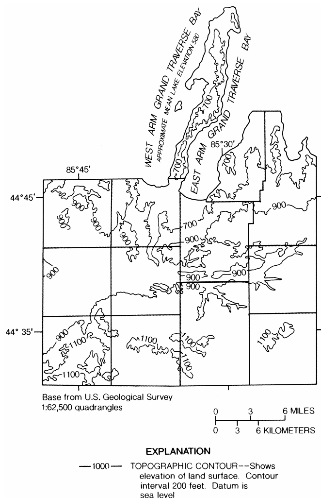
Figure 2.--Elevation of land surface.
