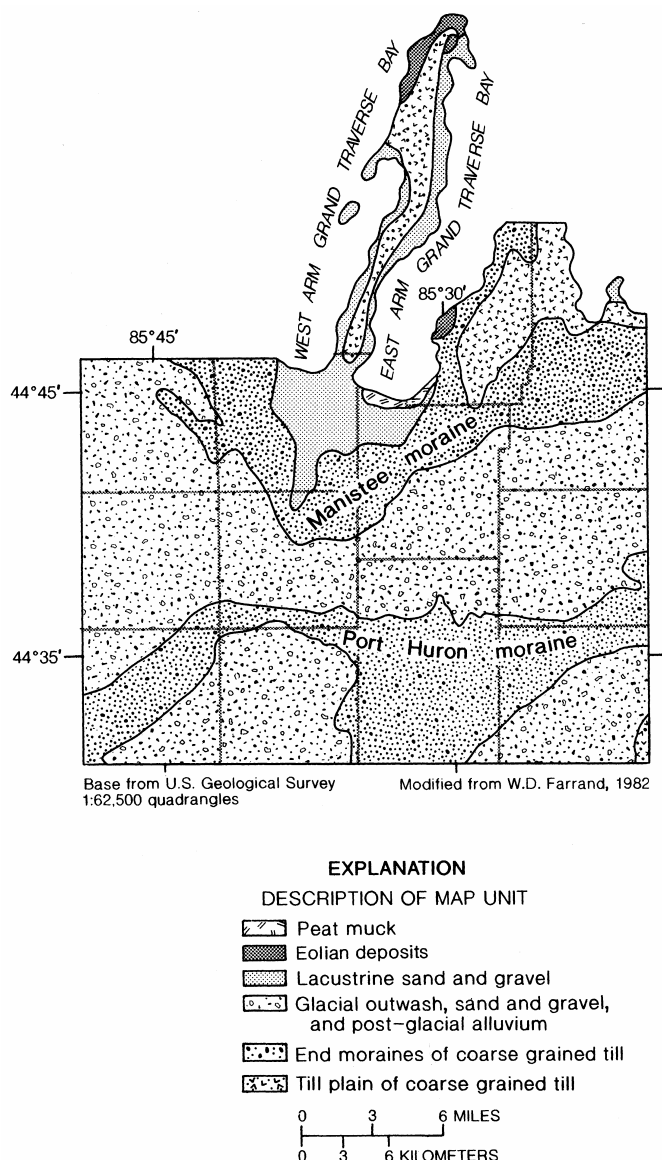
Figure 6.--Areal distribution of glacial deposits.
