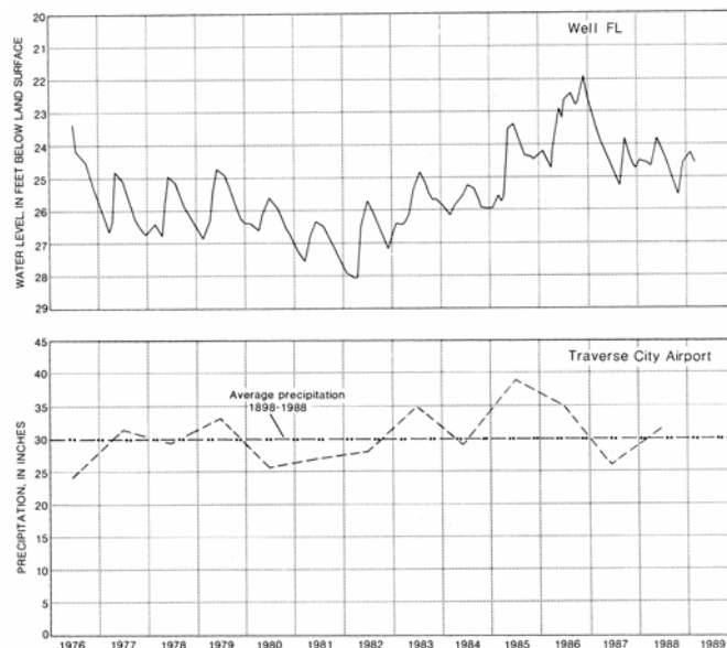
Figure 10.--Water-level fluctuations in observation well FL near Fife Lake, 1976-88, and annual precipitation at the Traverse City Airport, 1976-88.
