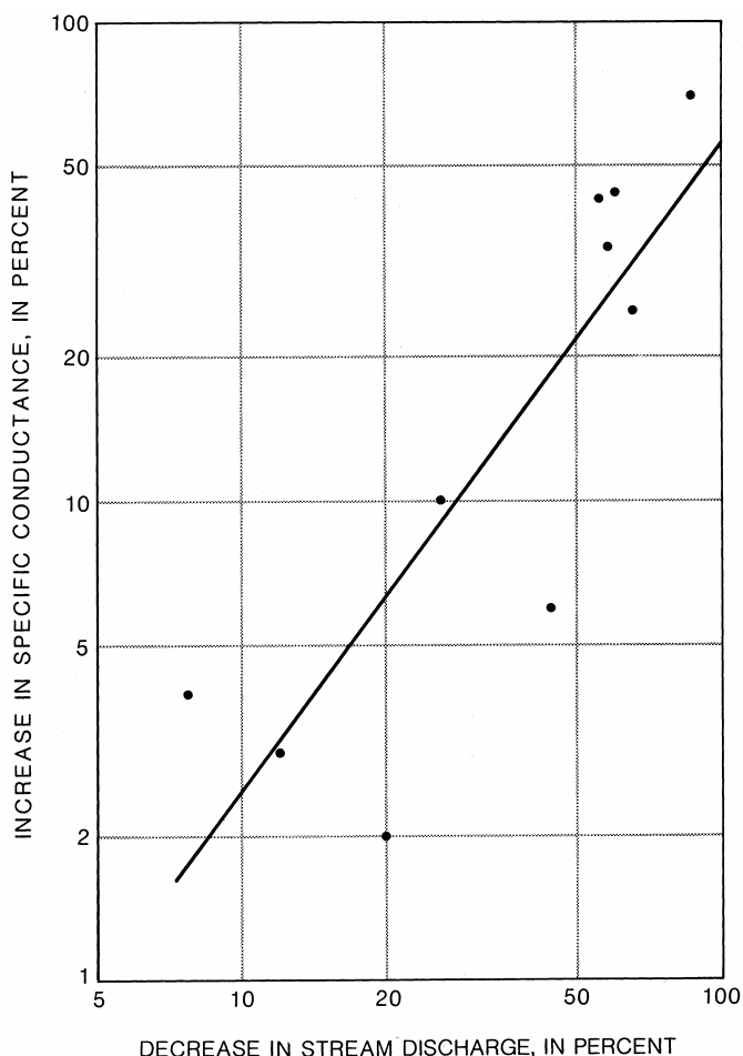
Figure 13.--Relation of specific conductance to stream discharge.
