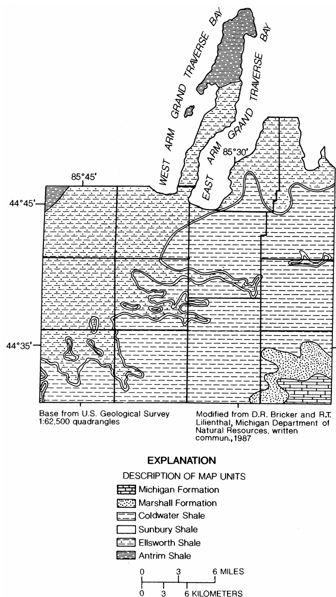
Figure 4.--Areal distribution of bedrock.
