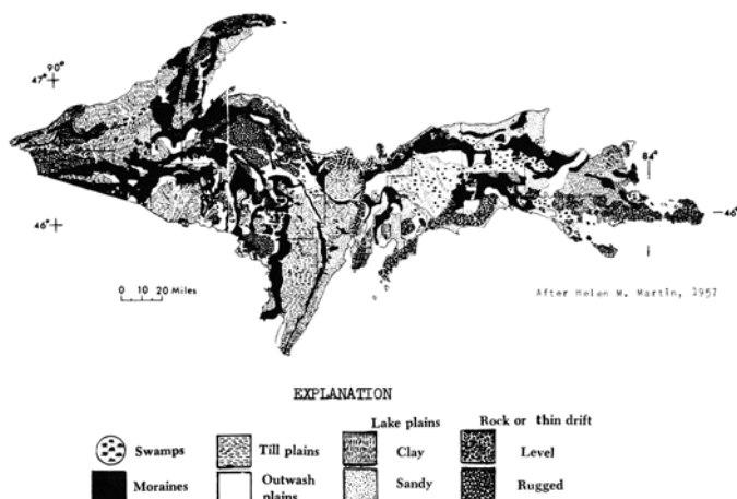
Figure 5.--Surficial geology influences streamflow.
