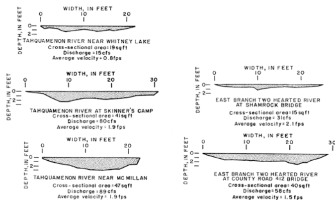
Figure 9.--Cross-sectional area and discharge of streams generally increase downstream.
