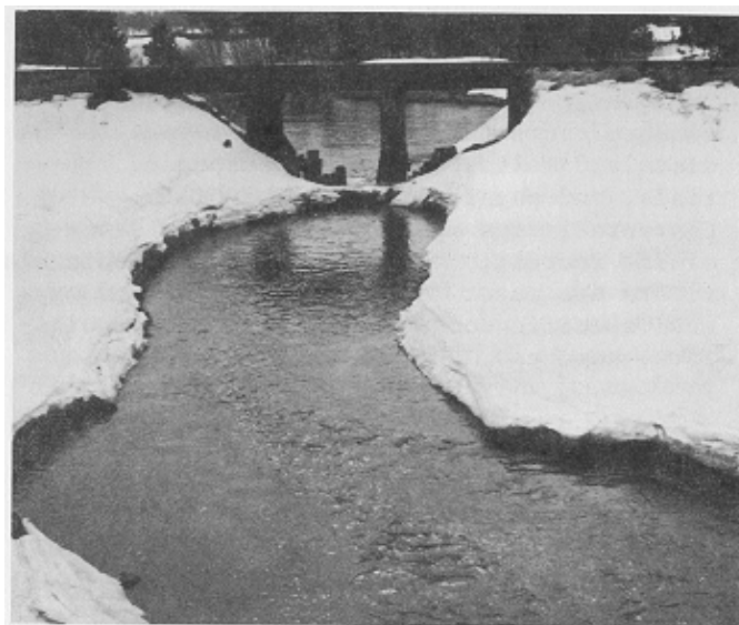
Figure 20.--Streams with a large component of ground-water inflow remain ice-free in winter.
