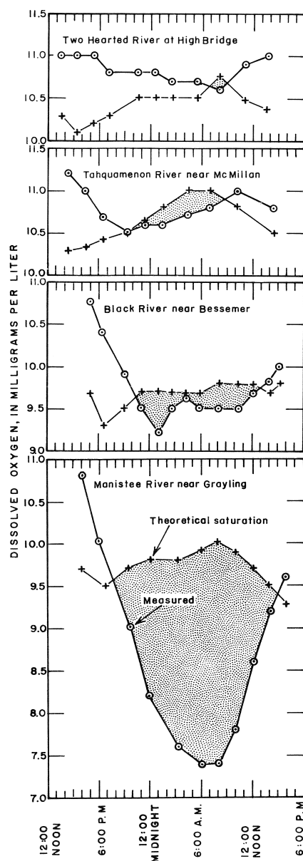
Figure 22.--Dissolved oxygen increases during daylight hours because of oxygen given off by plant photosynthesis. Diurnal
