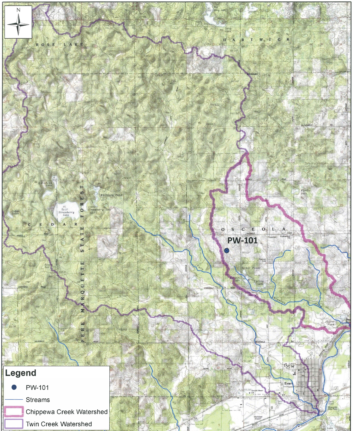
Figure 3.7 Chippewa Creek and Twin Creek Watersheds White Pine Springs, Osceola County, MI
