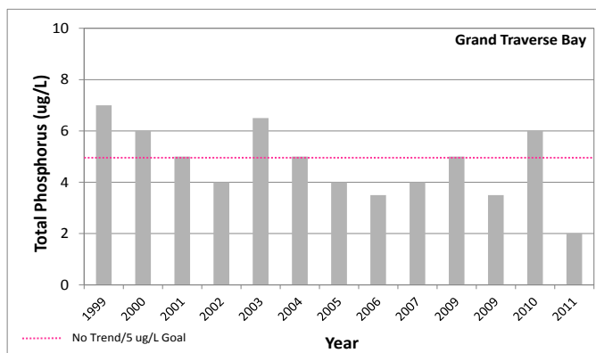
Figure 1. Annual Grand Traverse Bay total phosphorus concentrations and the WRD 5 µg/L total phosphorus metric.
