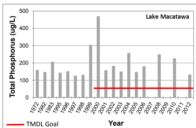
Figure 4. Lake Macatawa average spring total phosphorus concentrations and the total phosphorus TMDL goal of 50 µg/L.
