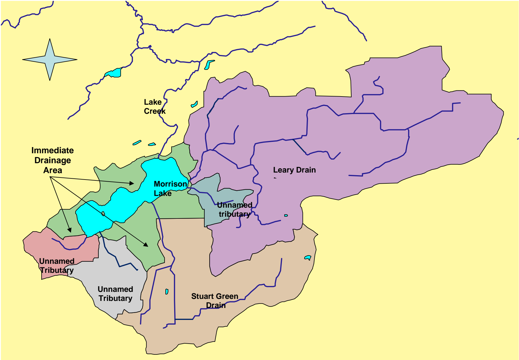
Figure 2. Morrison Lake sub-basin watersheds (Lesmez, 2008).
