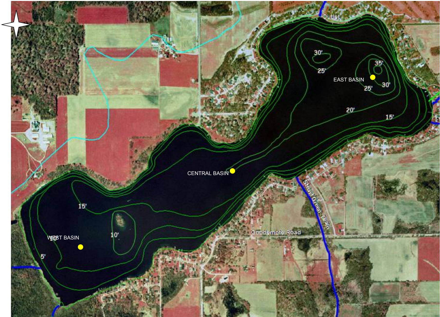
Figure 1. Morrison Lake contours, depth as feet, Ionia County, Michigan.
