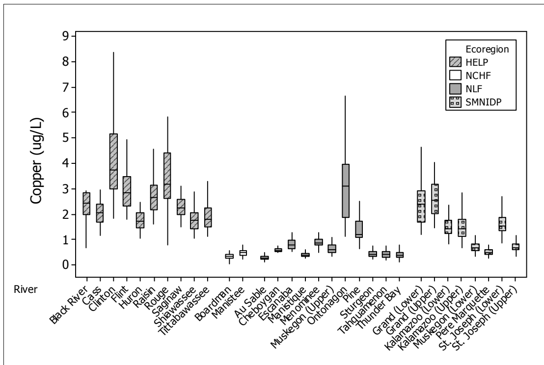
Figure 27. Median copper concentrations at WCMP tributary stations from 2000-2008. Results are categorized alphabetically by ecoregion.
