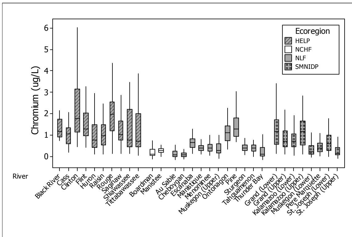
Figure 25. Median chromium concentrations at WCOMP tributary monitoring stations from 2000-2008. Results are categorized alphabetically by ecoregion.
