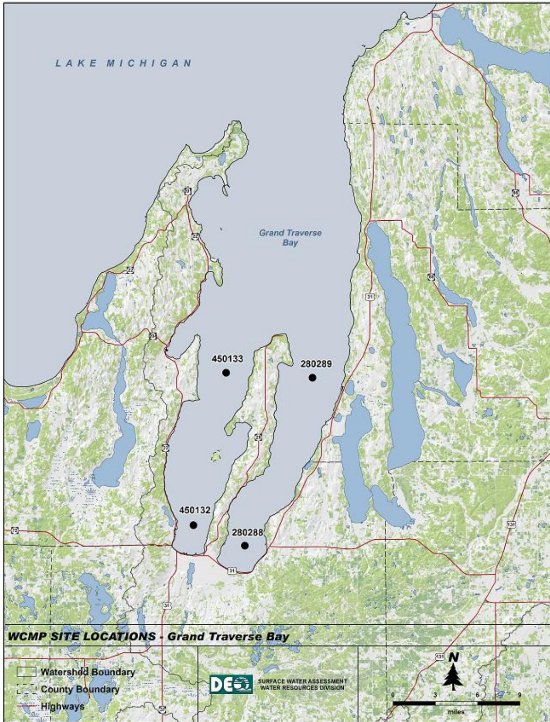
Figure 33. WCMC Monitoring locations, shown with STORET numbers, on Grand Traverse Bay; an embayment of Lake Michigan.
