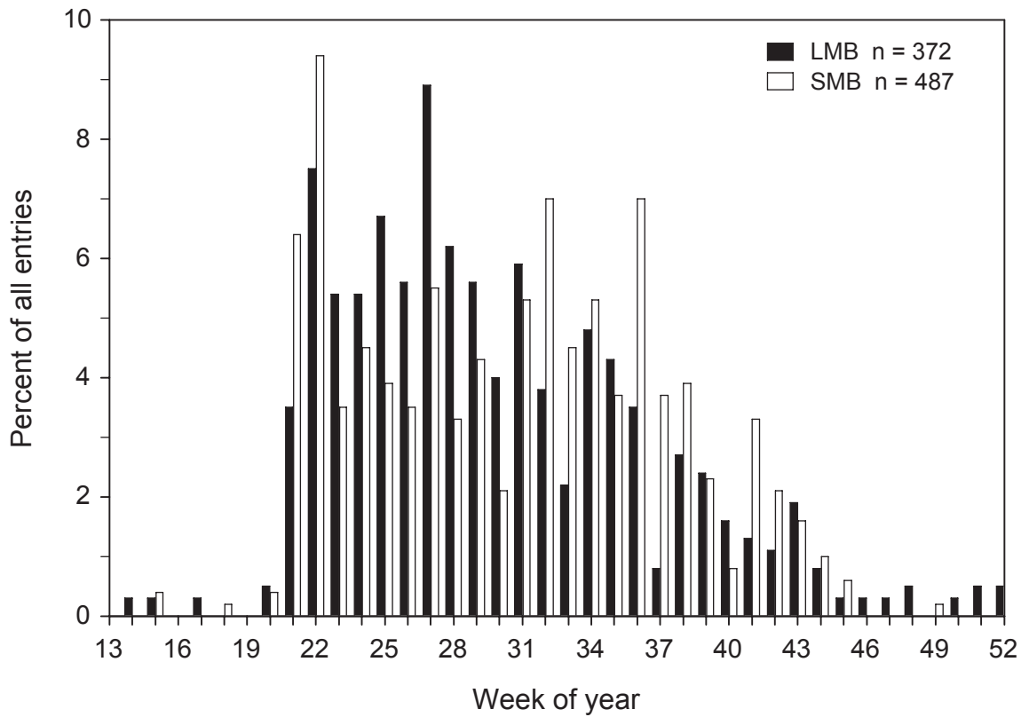
Figure 2.—Percent of all largemouth and smallmouth bass Master Angler entries for each week from 1992 through 2002. During this time period legal bass fishing began the Saturday of Memorial Day weekend (during the 21st week of the year) in the majority of the state’s waters.
