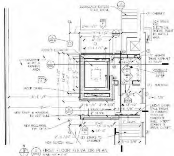
Figure 2: Plan of the Elevator Addition.
