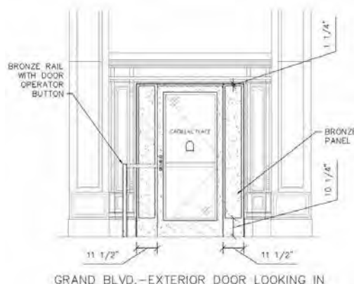
Figure 1: Elevation of new door centered in rotunda
