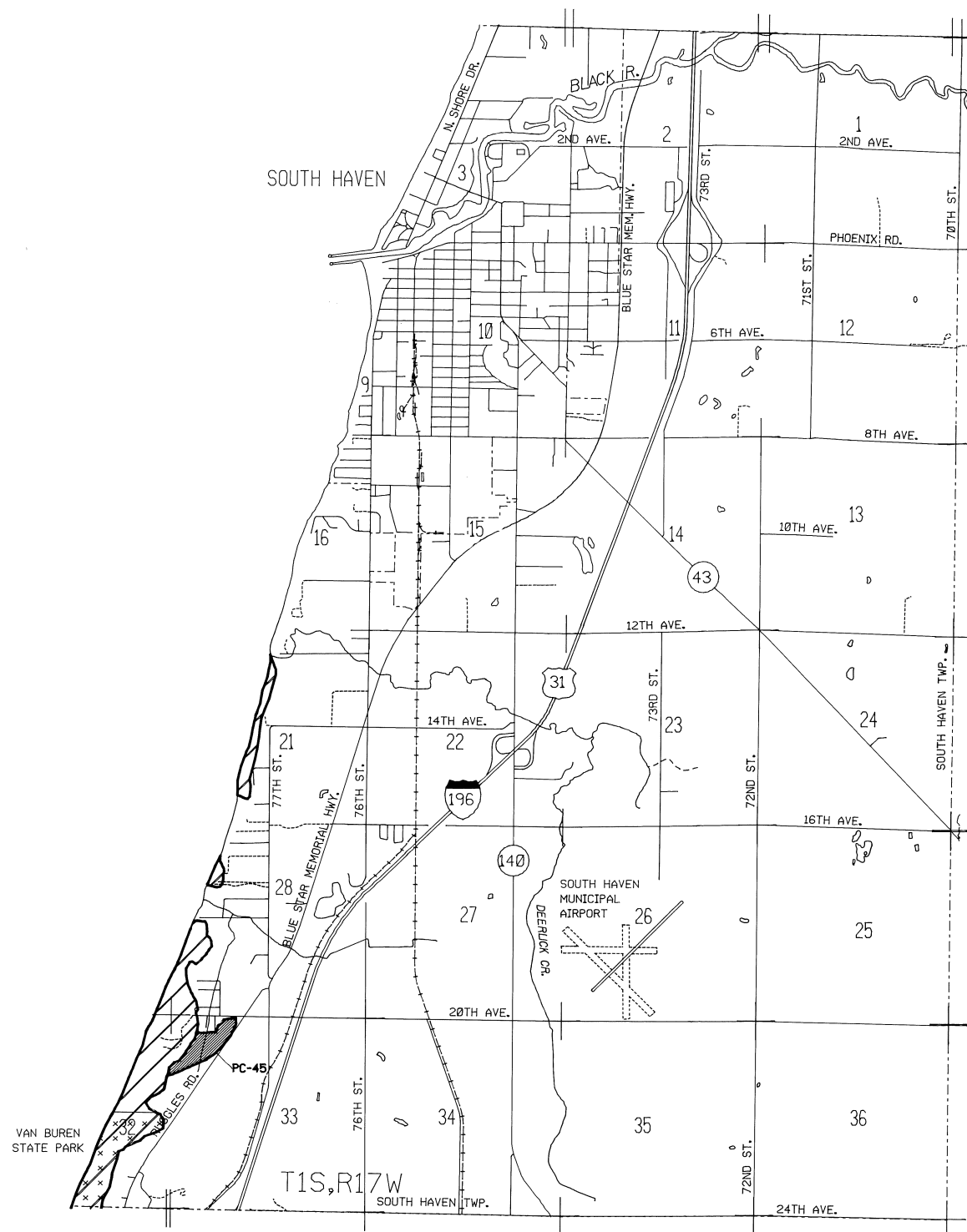
PC-45 - Mesic Southern Forest, Michigan Natural Features Inventory
