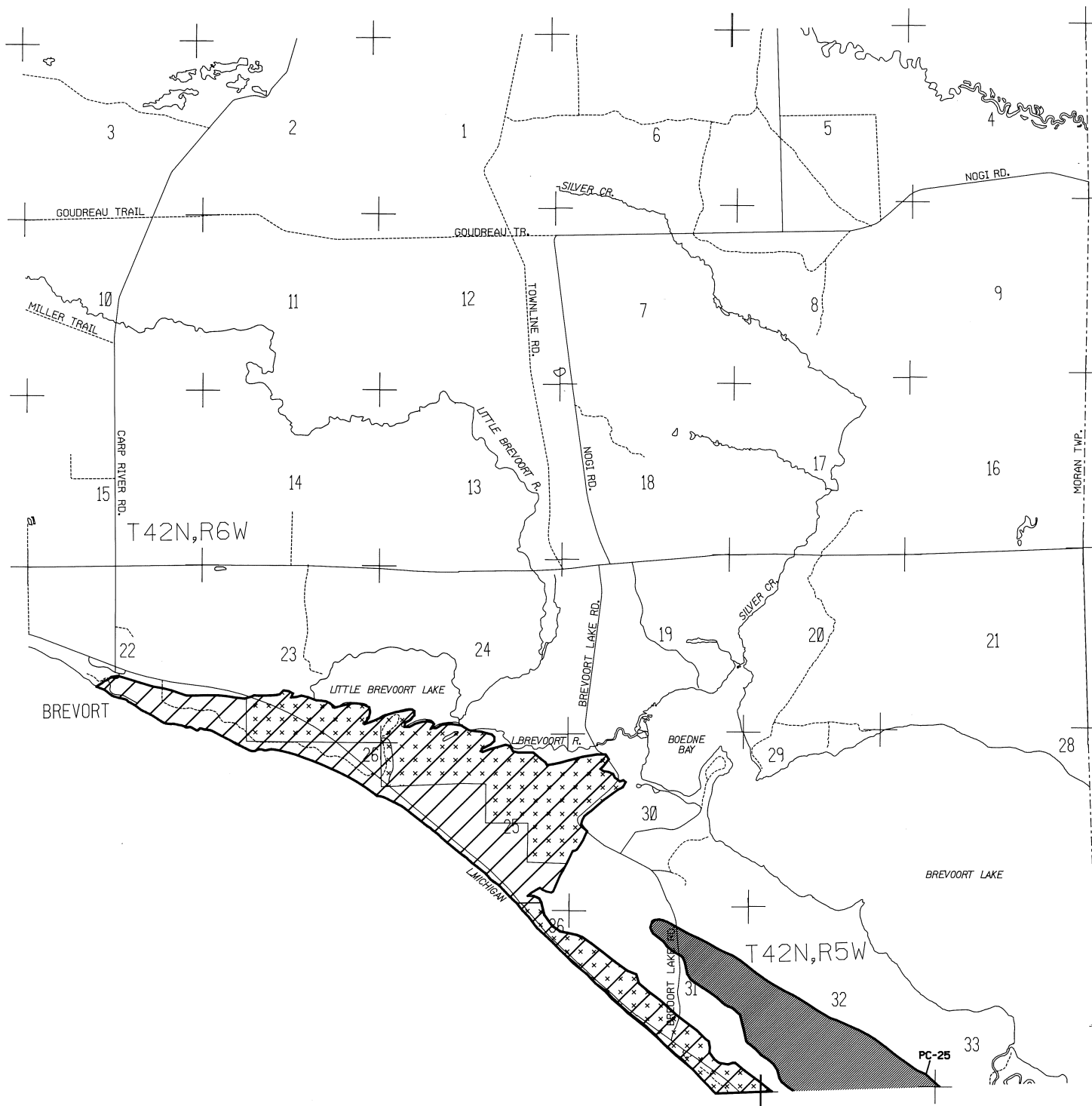
PC-25 - Wooded Dune and Swale Complex, Michigan Natural Features Inventory
