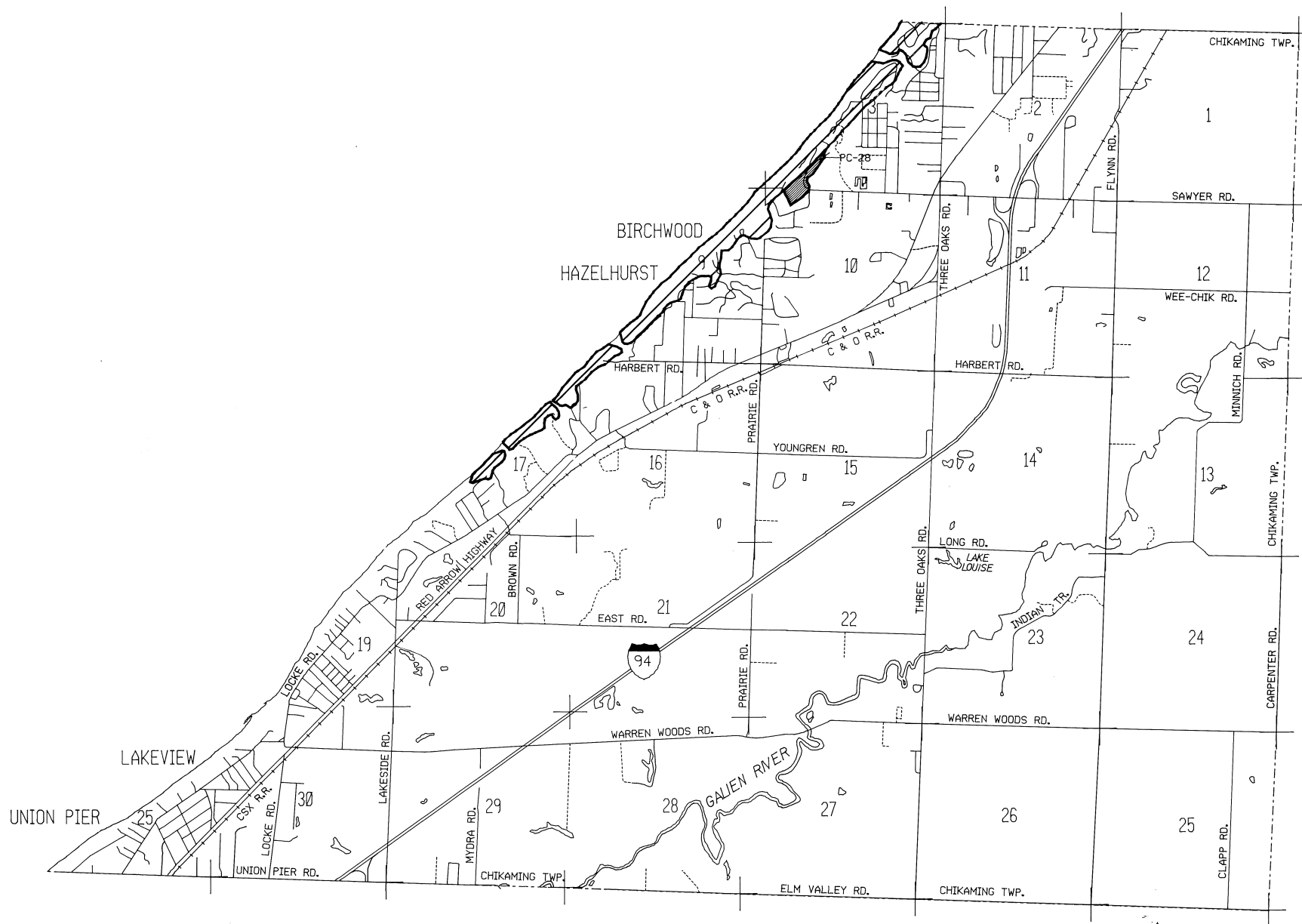
PC-28 - Dry-mesic Southern Forest, Michigan Natural Features Inventory
