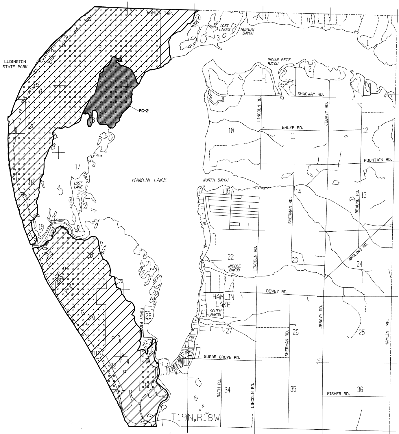
PC-2 - Open Dunes, Michigan Natural Features Inventory
