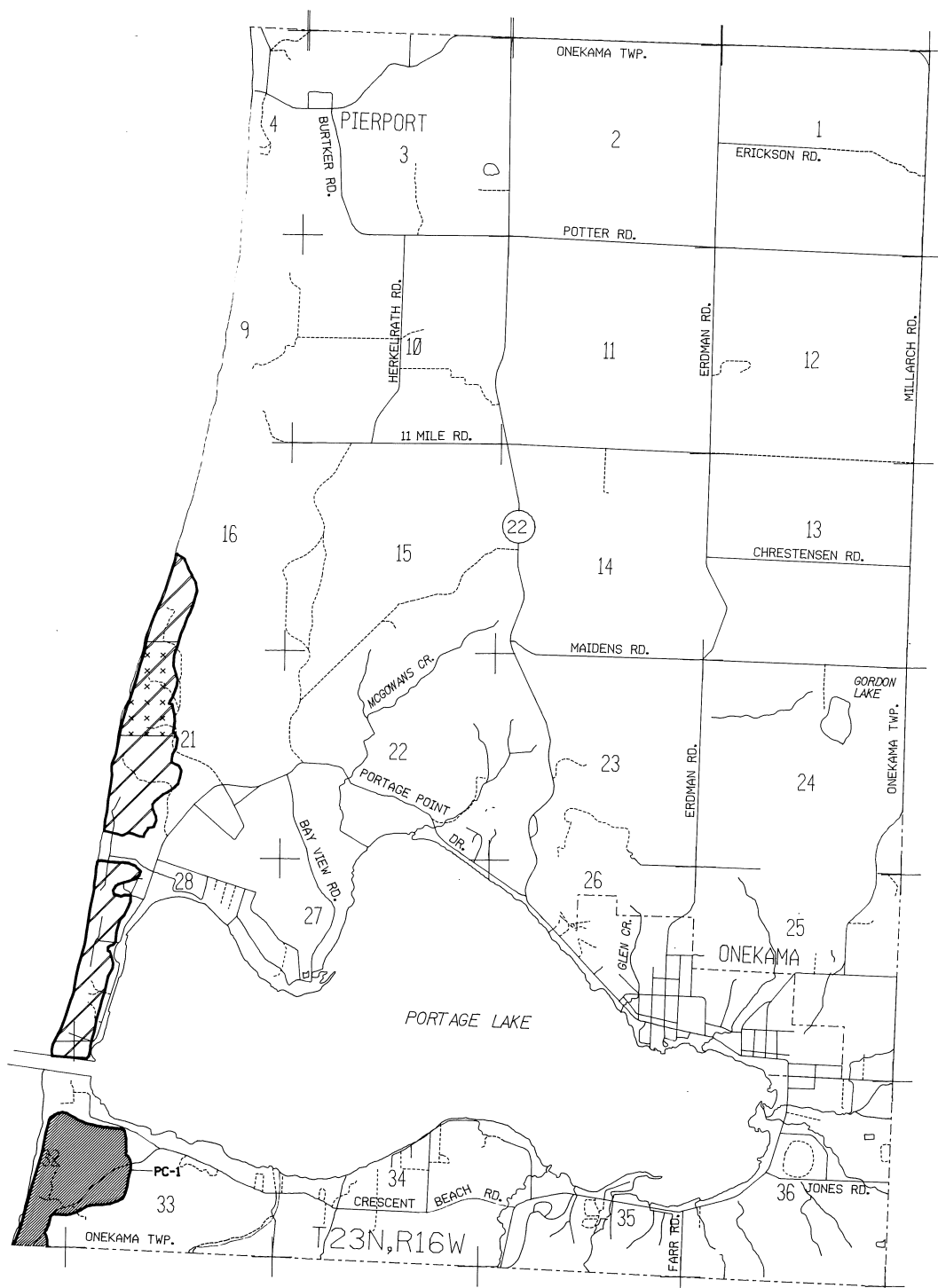
PC-1 - Mesic Northern Forest, Michigan Natural Features Inventory
