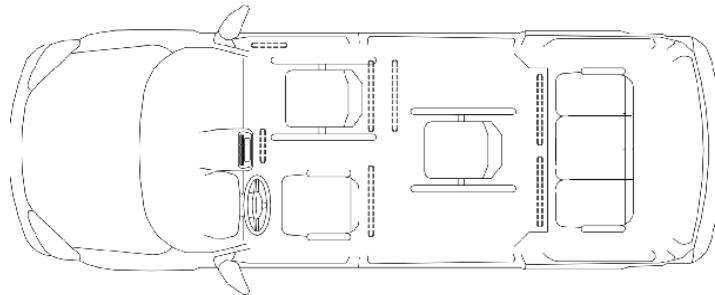
3+2 Modified Chassis Vehicle with ramp – vinyl (less double fold- away seat).
