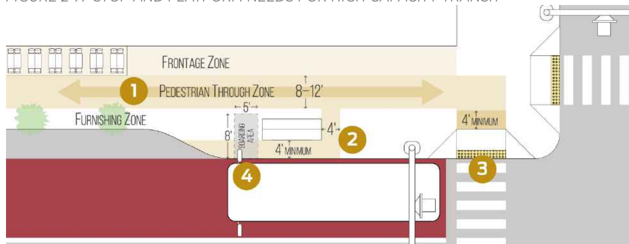
FIGURE 2-7: STOP AND PLATFORM NEEDS FOR HIGH CAPACITY TRANSIT
