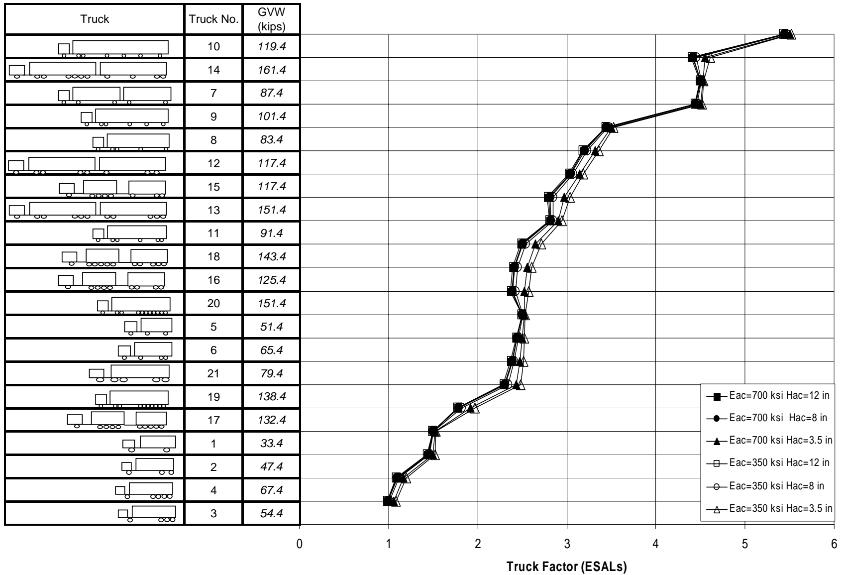
Figure 2 Fatigue-based Truck Factors within AASHTO LEF framework
