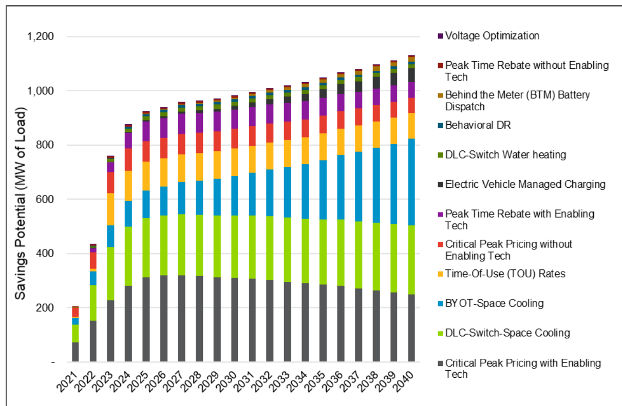
Figure 3-7. Lower Peninsula Electric Summer Residential Potential by DR Suboption (MW at Meter)
