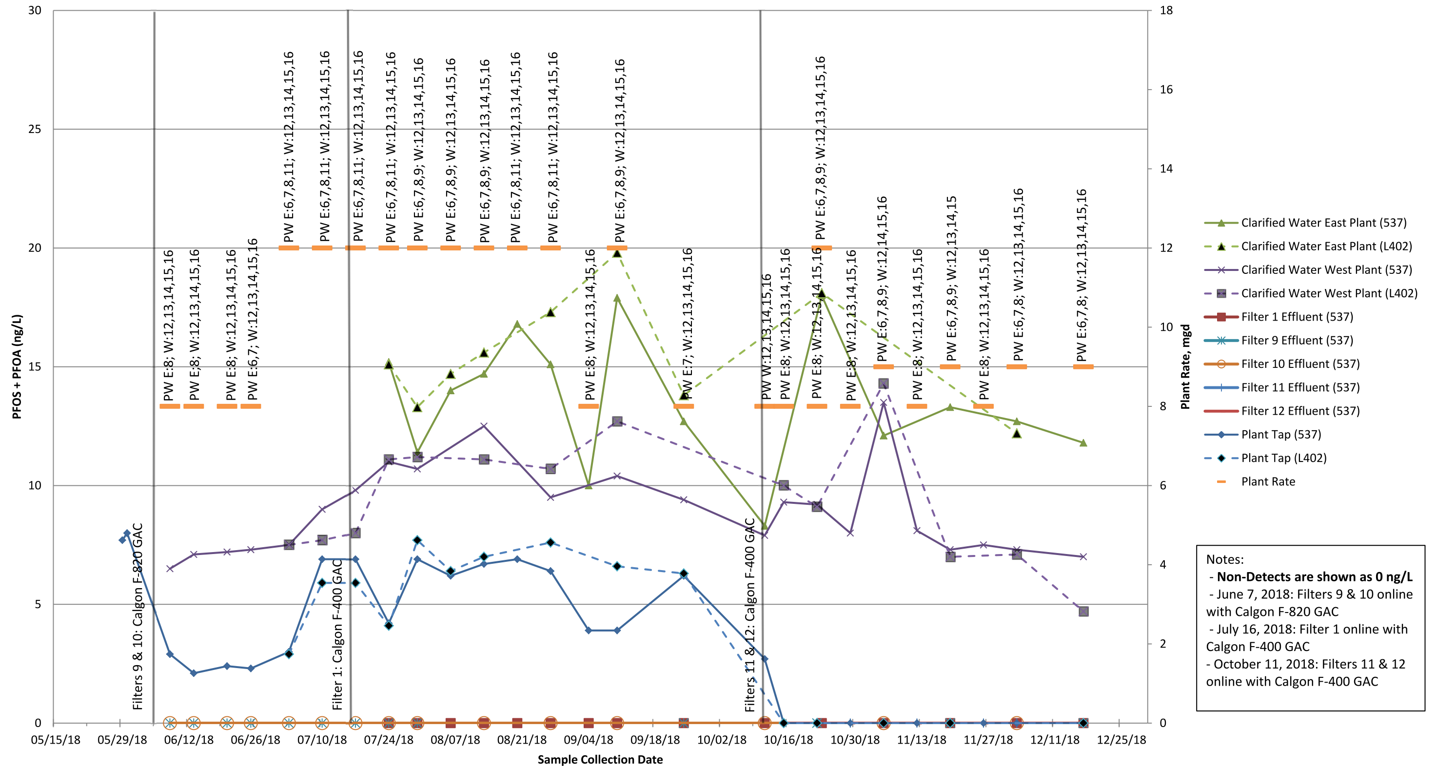
Plainfield Water Treatment Plant - Filter GAC Pilot Study FIGURE 1 - PFOS + PFOA, EPA Method 537 vs L402
