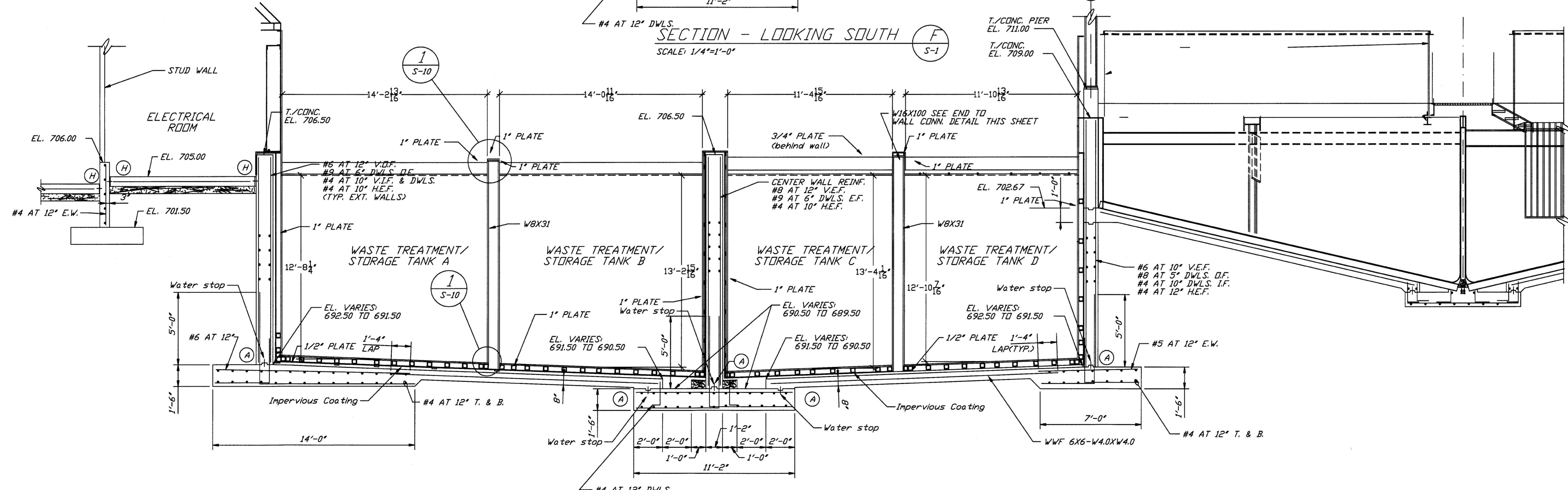
SECTION - LOOKING NORTH SCALE: 1/4"=1'-0"
