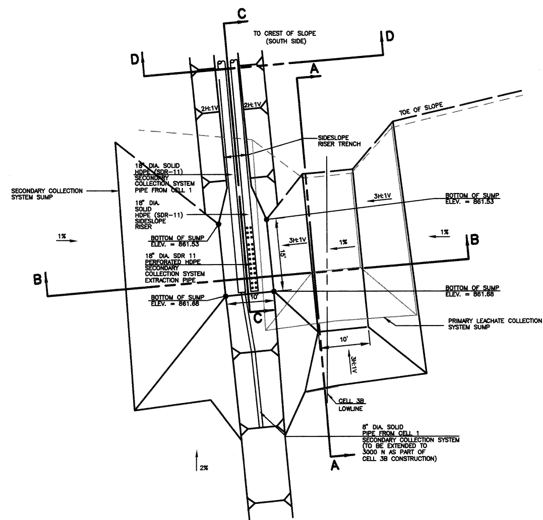
CELL 3B SECONDARY COLLECTION SYSTEM SUMP PLAN NOT TO SCALE
