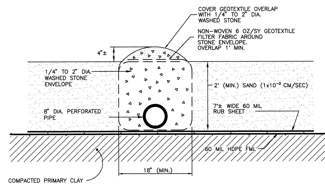
PRIMARY LEACHATE COLLECTION PIPE SYSTEM DETAIL NOT TO SCALE
