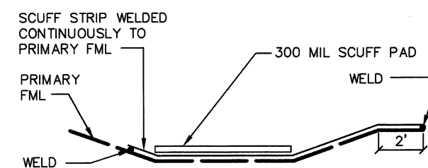
TYPICAL SUMP PAD/SCUFF STRIP CROSS SECTION NOT TO SCALE
