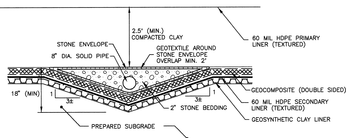
SECTION E-E CELL 1D SECONDARY COLLECTION TRENCH NOT TO SCALE
