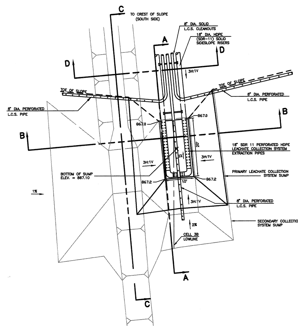
CELL 3B PRIMARY LEACHATE COLLECTION SYSTEM SUMP PLAN NOT TO SCALE
