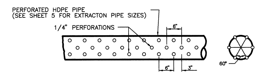
PIPE PERFORATION DETAIL FOR HDPE EXTRACTION PIPE NOT TO SCALE
