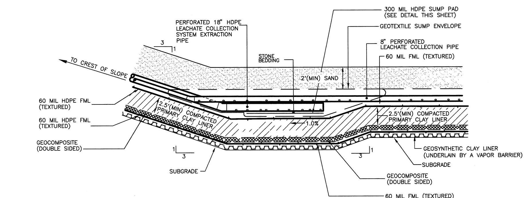
SUMP CROSS SECTION A-A NOT TO SCALE
