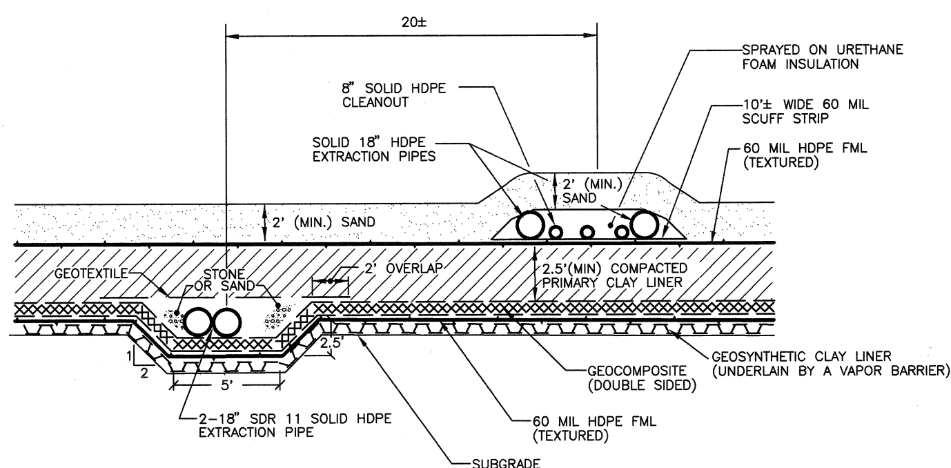
SECTION D-D SIDE SLOPE RISER TRENCH DETAIL NOT TO SCALE
