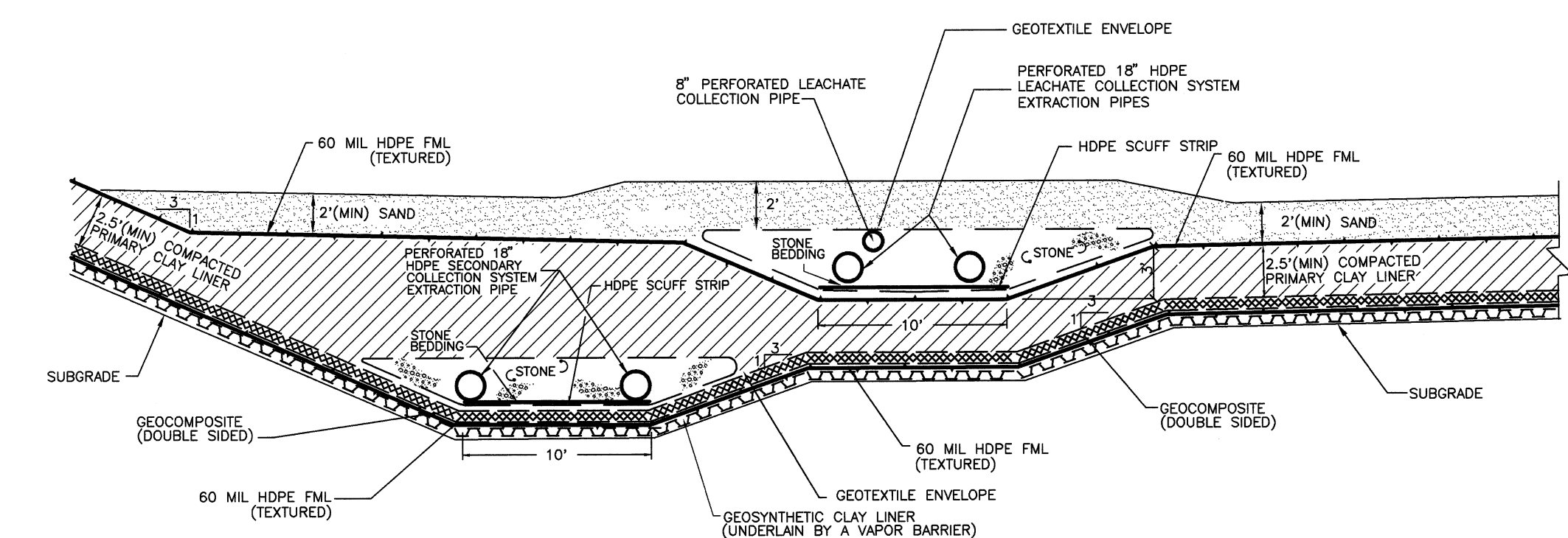
SUMP CROSS SECTION B-B NOT TO SCALE
