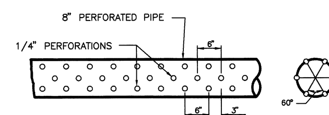
LEACHATE COLLECTION SYSTEM PIPE PERFORATION DETAIL NOT TO SCALE
