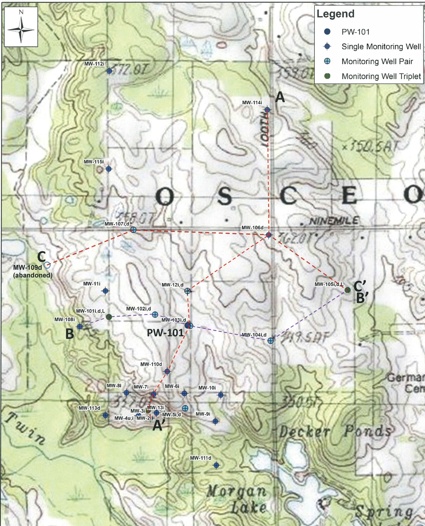
Figure 3.1a Location Map of Monitoring Wells and Cross Sections White Pine Springs, Osceola County, MI
