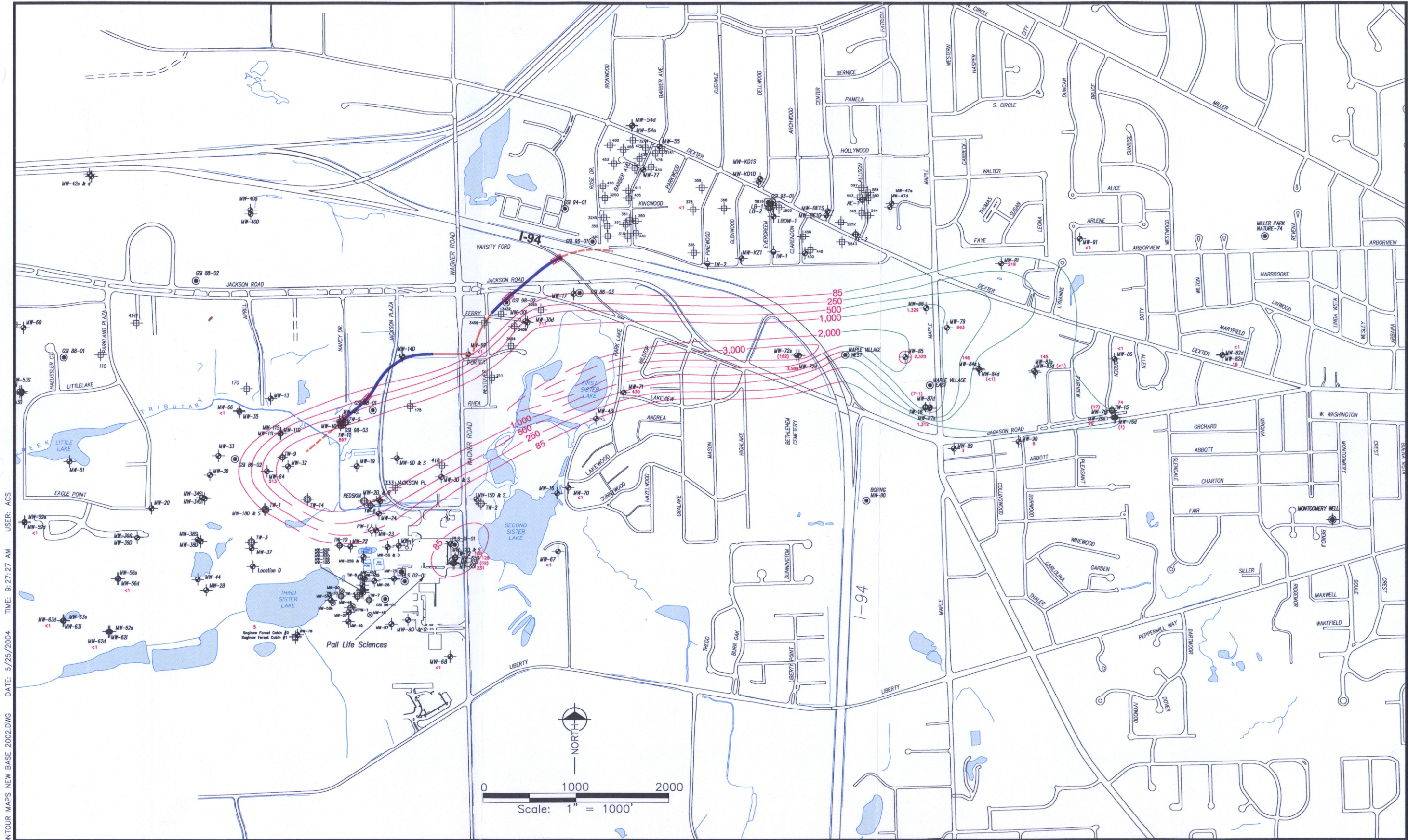
UNIT E AQUIFER 1,4-DIOXANE ISOCONCENTRATION MAP JANUARY-MARCH 2004
