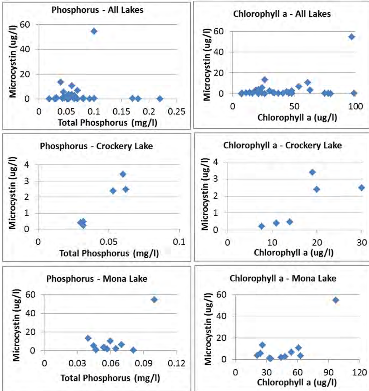
Figure 4(a). Total phosphorus (mg/L) and chlorophyll a vs average microcystin ( \mu\text{g/L} ) concentrations. Each data point is 1 sample date. The top graphs present the data for all lakes, followed by the data for Crockery and Mona Lakes. NOTE: One outlier chlorophyll a data point (Morrison Lake: 350 \mu\text{g/L} chlorophyll a and 0.26 \mu\text{g/L} total microcystin) was removed from the all lakes graph.
