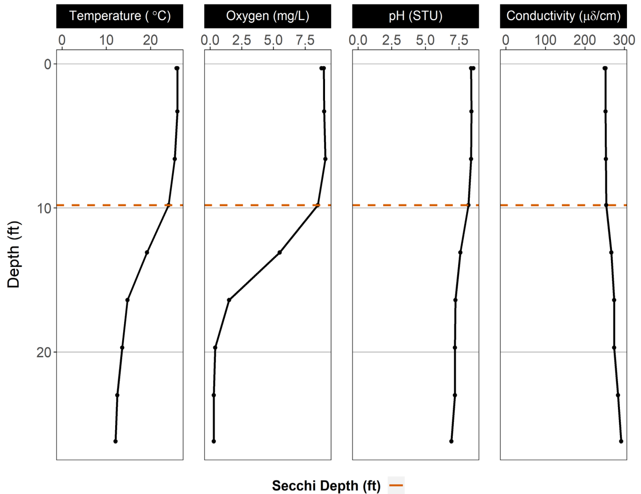
Figure 2. Vertical profile of temperature, dissolved oxygen, pH, and conductivity collected during the 2017 National Lakes Assessment of Saddle Lake.
