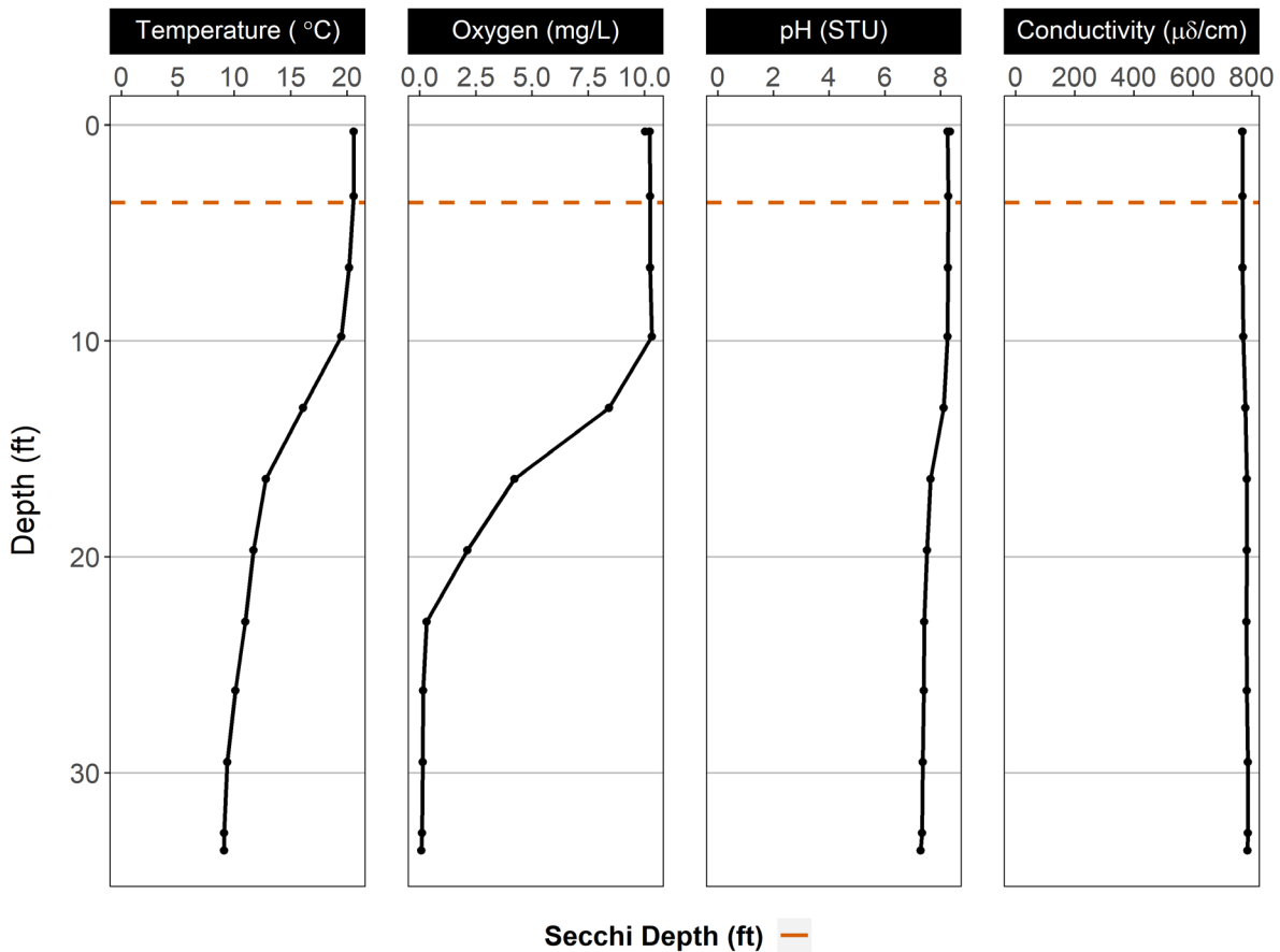
Figure 2. Vertical profile of temperature, dissolved oxygen, pH, and conductivity collected during the 2017 National Lakes Assessment of Bogie Lake.
