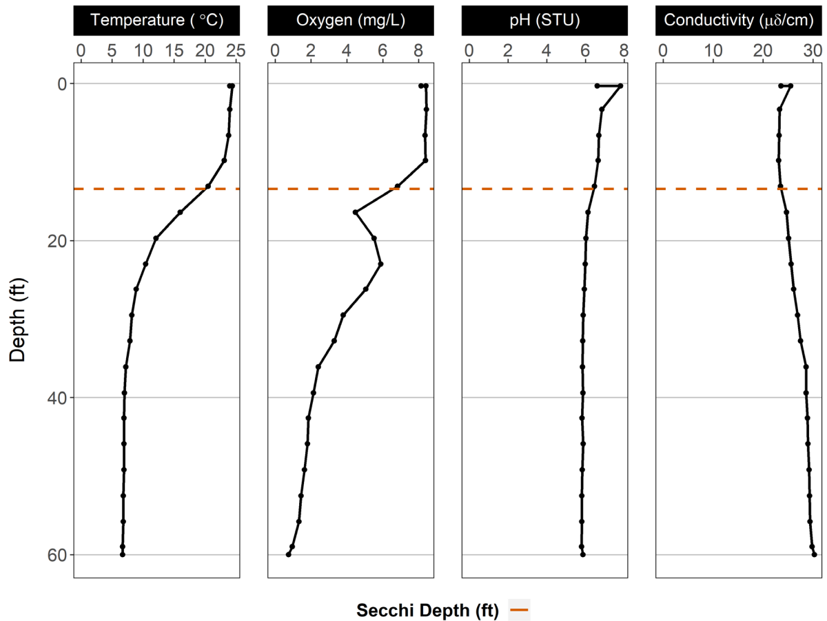
Figure 2. Vertical profile of temperature, dissolved oxygen, pH, and conductivity collected during the 2017 National Lakes Assessment of Silver Lake.
