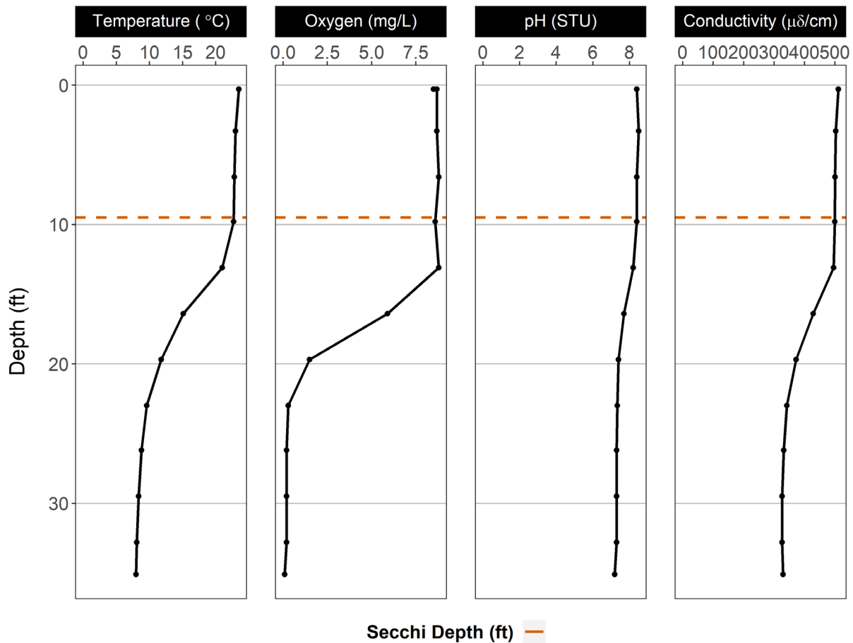
Figure 2. Vertical profile of temperature, dissolved oxygen, pH, and conductivity collected during the 2017 National Lakes Assessment of Tupper Lake.
