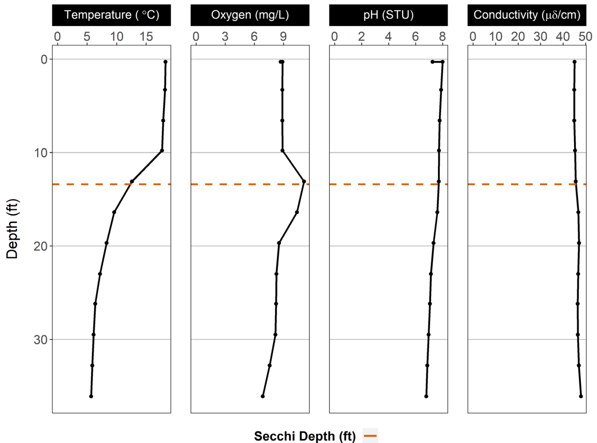
Figure 2. Vertical profile of temperature, dissolved oxygen, pH, and conductivity collected during the 2017 National Lakes Assessment of Lake Alice.
