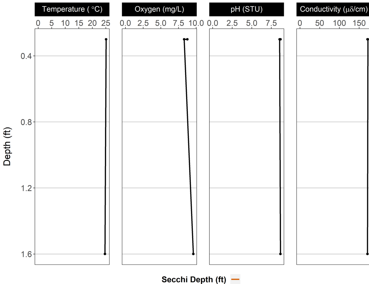
Figure 2. Vertical profile of temperature, dissolved oxygen, pH, and conductivity collected during the 2017 National Lakes Assessment of Lorraine Lake.
