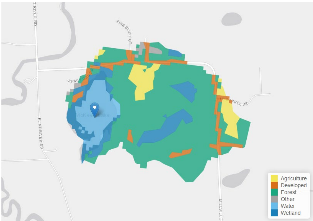
Figure 1. Land use map of McKeen Lake.
