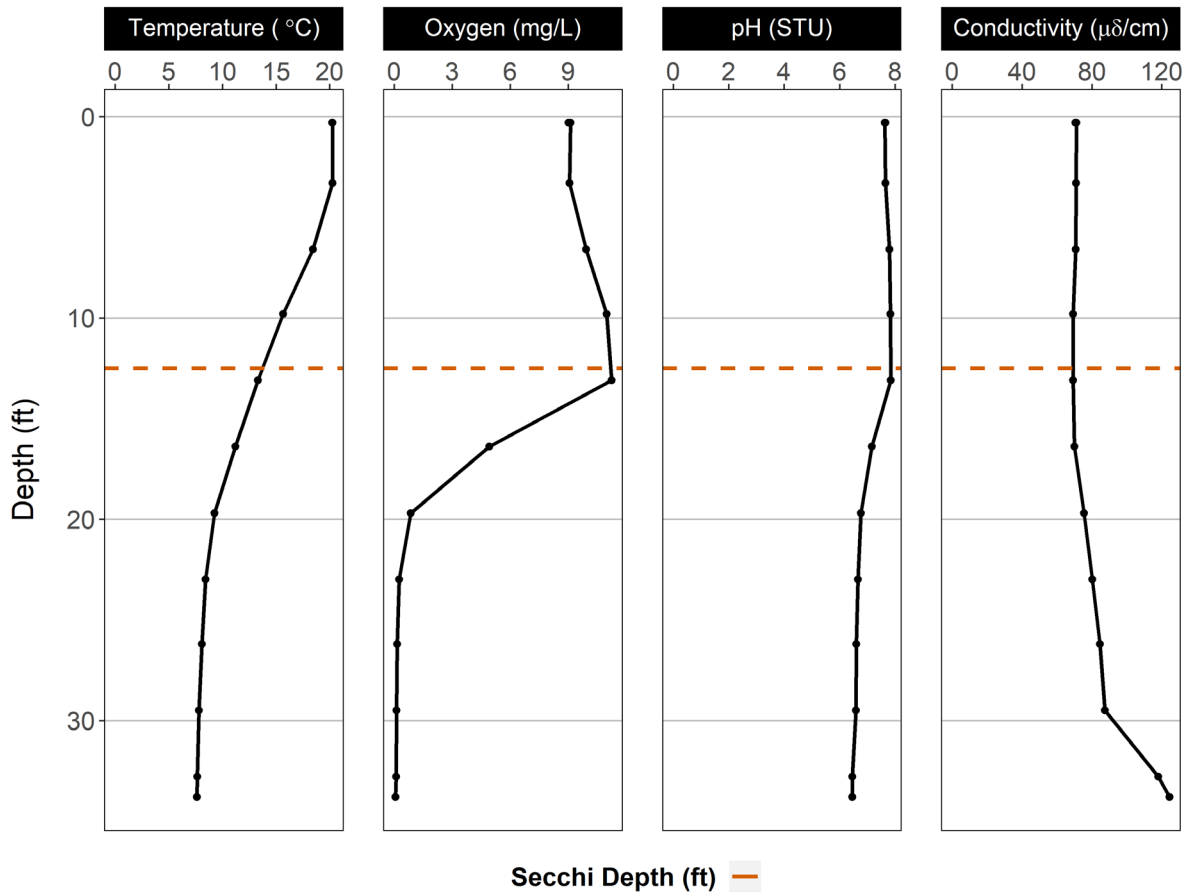
Figure 2. Vertical profile of temperature, dissolved oxygen, pH, and conductivity collected during the 2017 National Lakes Assessment of McKean Lake.
