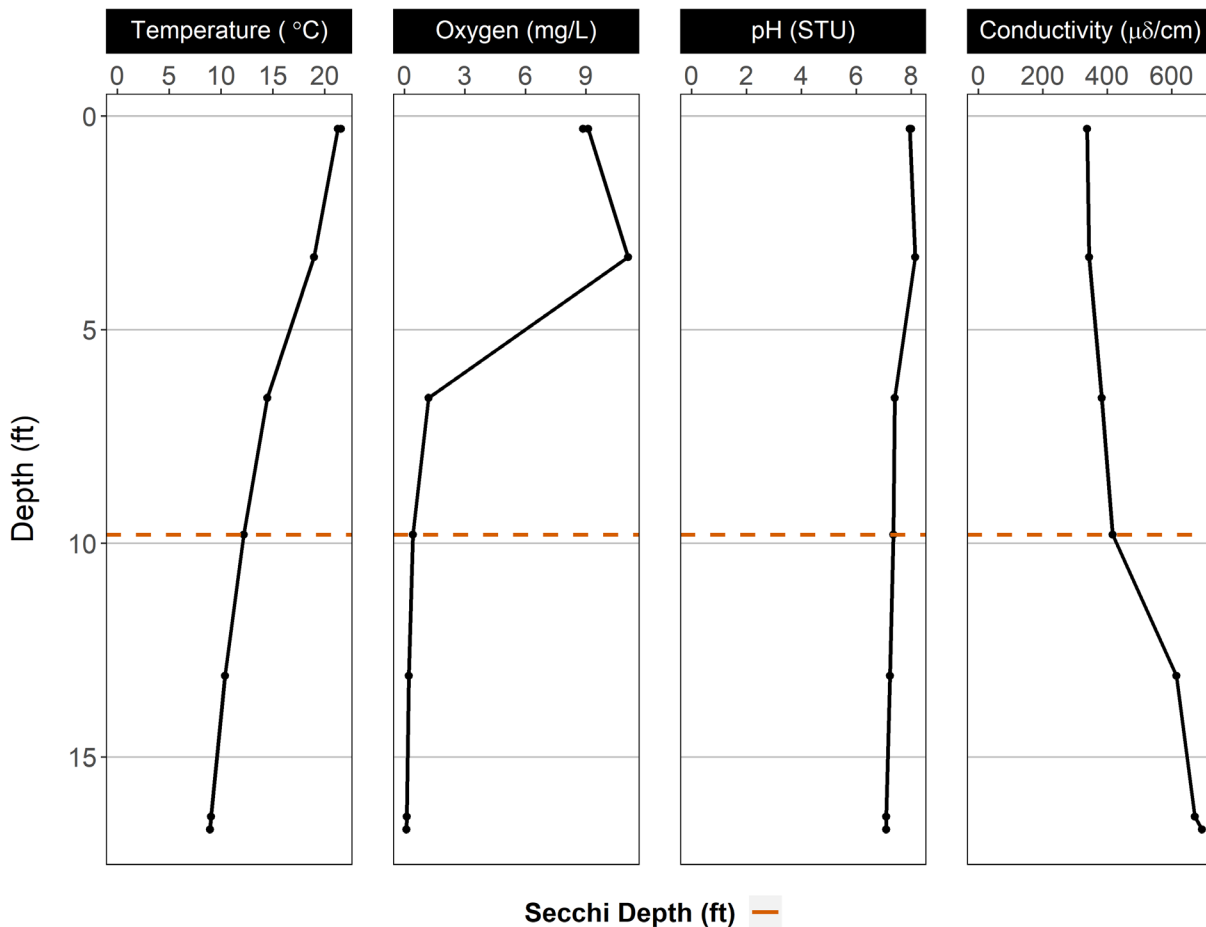
Figure 2. Vertical profile of temperature, dissolved oxygen, pH, and conductivity collected during the 2017 National Lakes Assessment of Rollway Lake.
