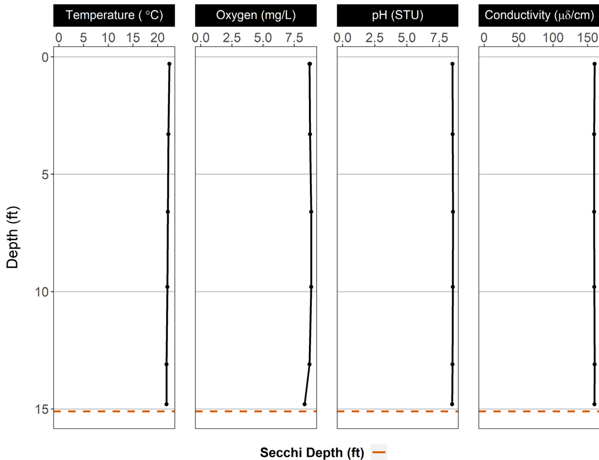
Figure 2. Vertical profile of temperature, dissolved oxygen, pH, and conductivity collected during the 2017 National Lakes Assessment of Crystal Lake.
