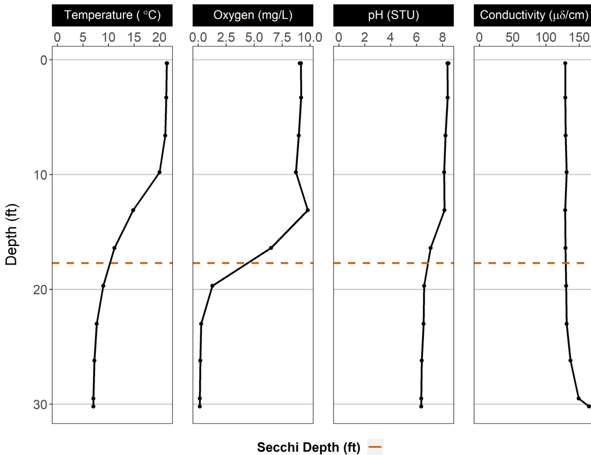
Figure 2. Vertical profile of temperature, dissolved oxygen, pH, and conductivity collected during the 2017 National Lakes Assessment of Blaine Lake.
