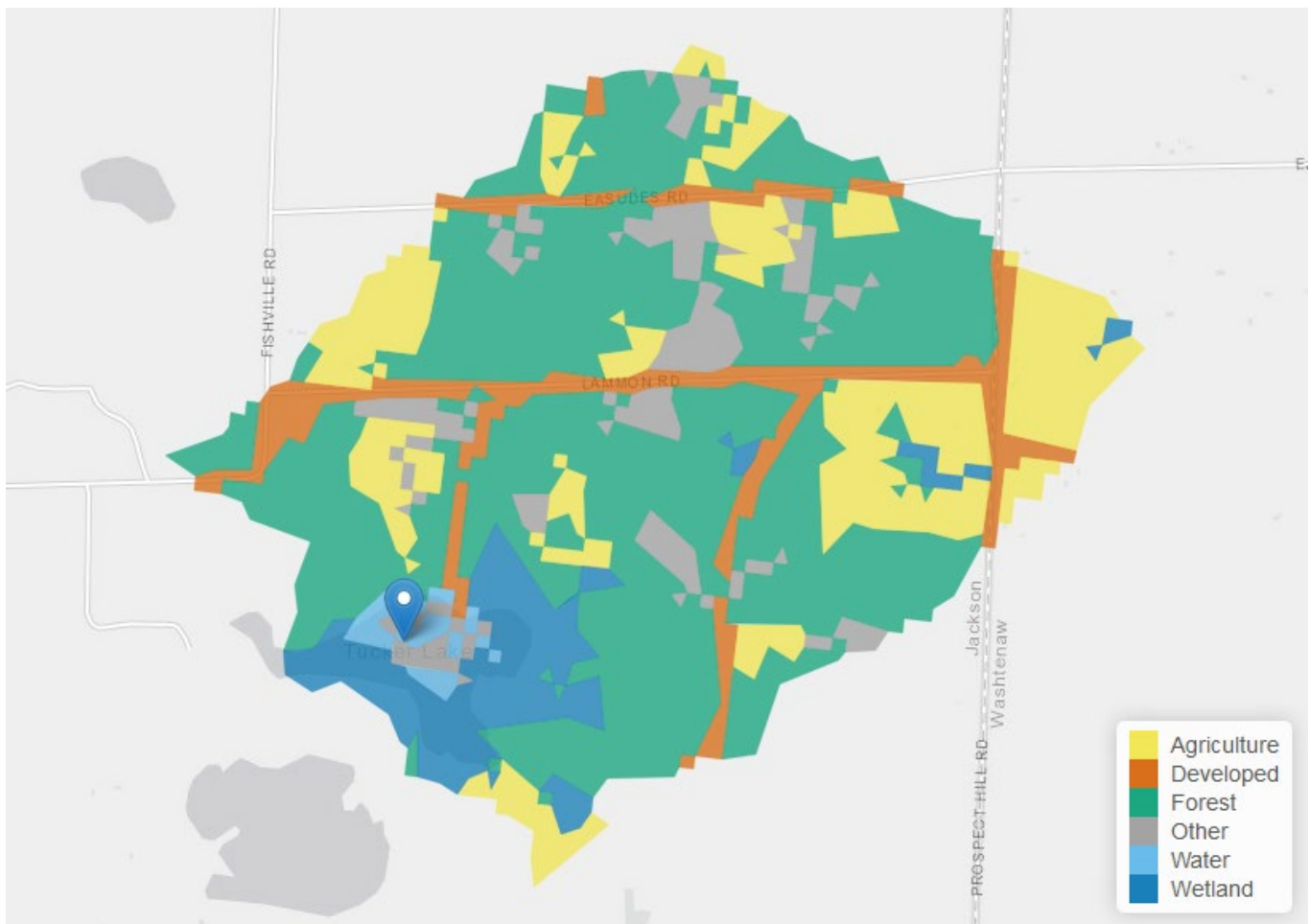
Figure 1. Land use map of Tucker Lake.
