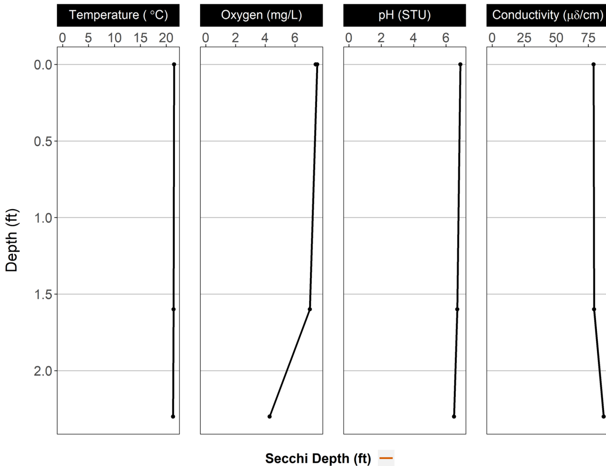
Figure 2. Vertical profile of temperature, dissolved oxygen, pH, and conductivity collected during the 2017 National Lakes Assessment of Tucker Lake.
