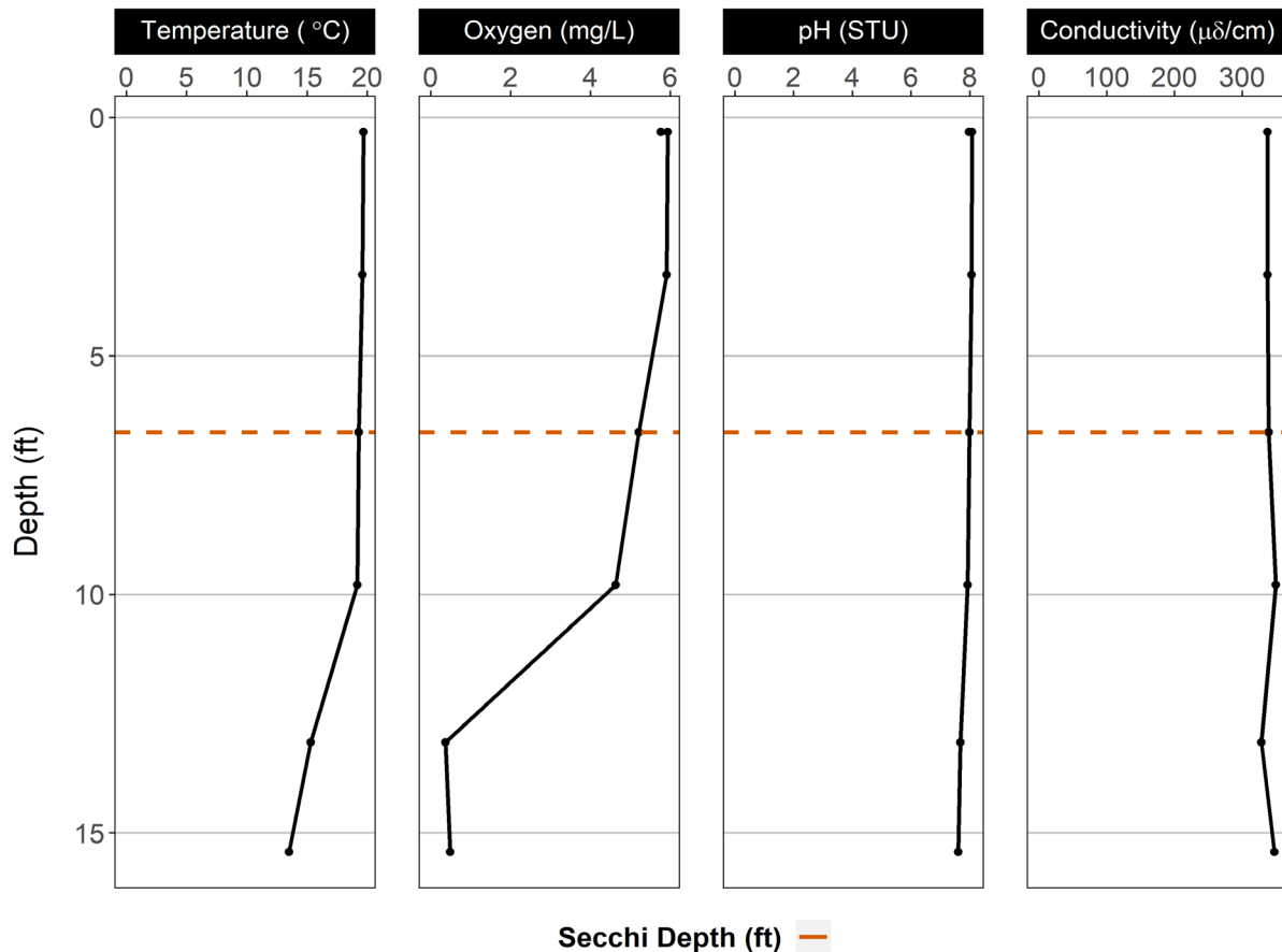
Figure 2. Vertical profile of temperature, dissolved oxygen, pH, and conductivity collected during the 2017 National Lakes Assessment of Sherrett Lake.
