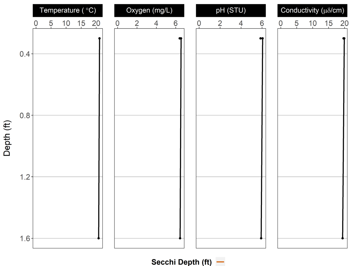
Figure 2. Vertical profile of temperature, dissolved oxygen, pH, and conductivity collected during the 2017 National Lakes Assessment of Gilligan Lake.
