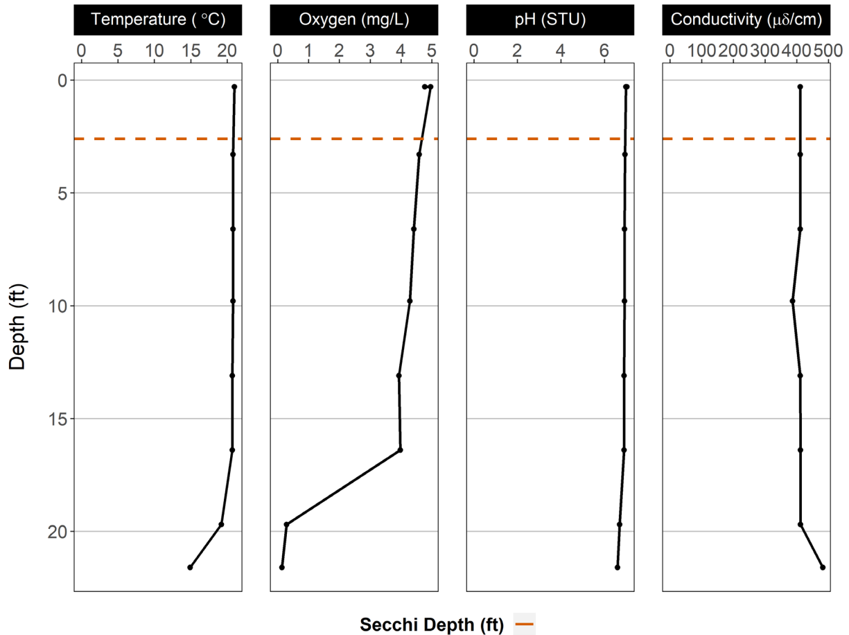
Figure 2. Vertical profile of temperature, dissolved oxygen, pH, and conductivity collected during the 2017 National Lakes Assessment of Wallace Lake.
