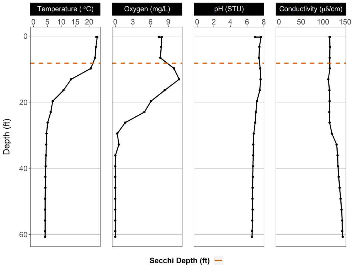
Figure 2. Vertical profile of temperature, dissolved oxygen, pH, and conductivity collected during the 2017 National Lakes Assessment of McAvoy Lake.
