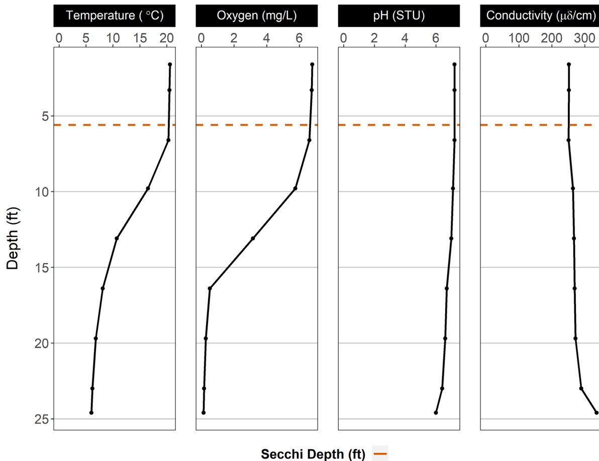
Figure 2. Vertical profile of temperature, dissolved oxygen, pH, and conductivity collected during the 2017 National Lakes Assessment of Anderson Lake.
