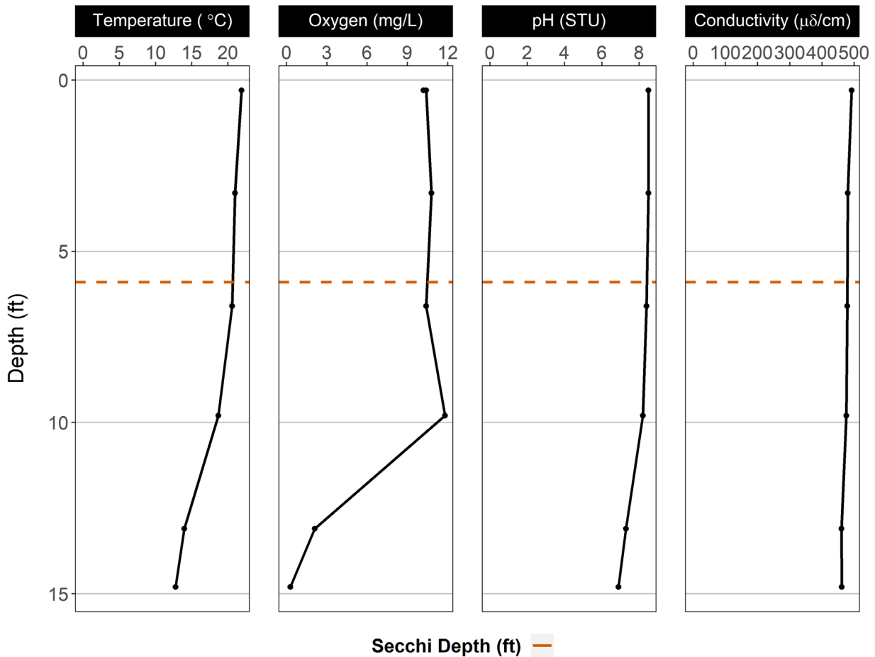
Figure 2. Vertical profile of temperature, dissolved oxygen, pH, and conductivity collected during the 2017 National Lakes Assessment of Tray Lake.
